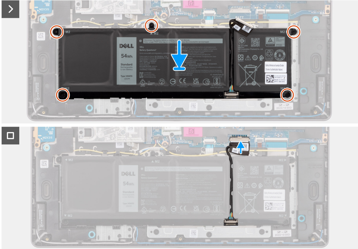
Figure 31. Installing the battery
