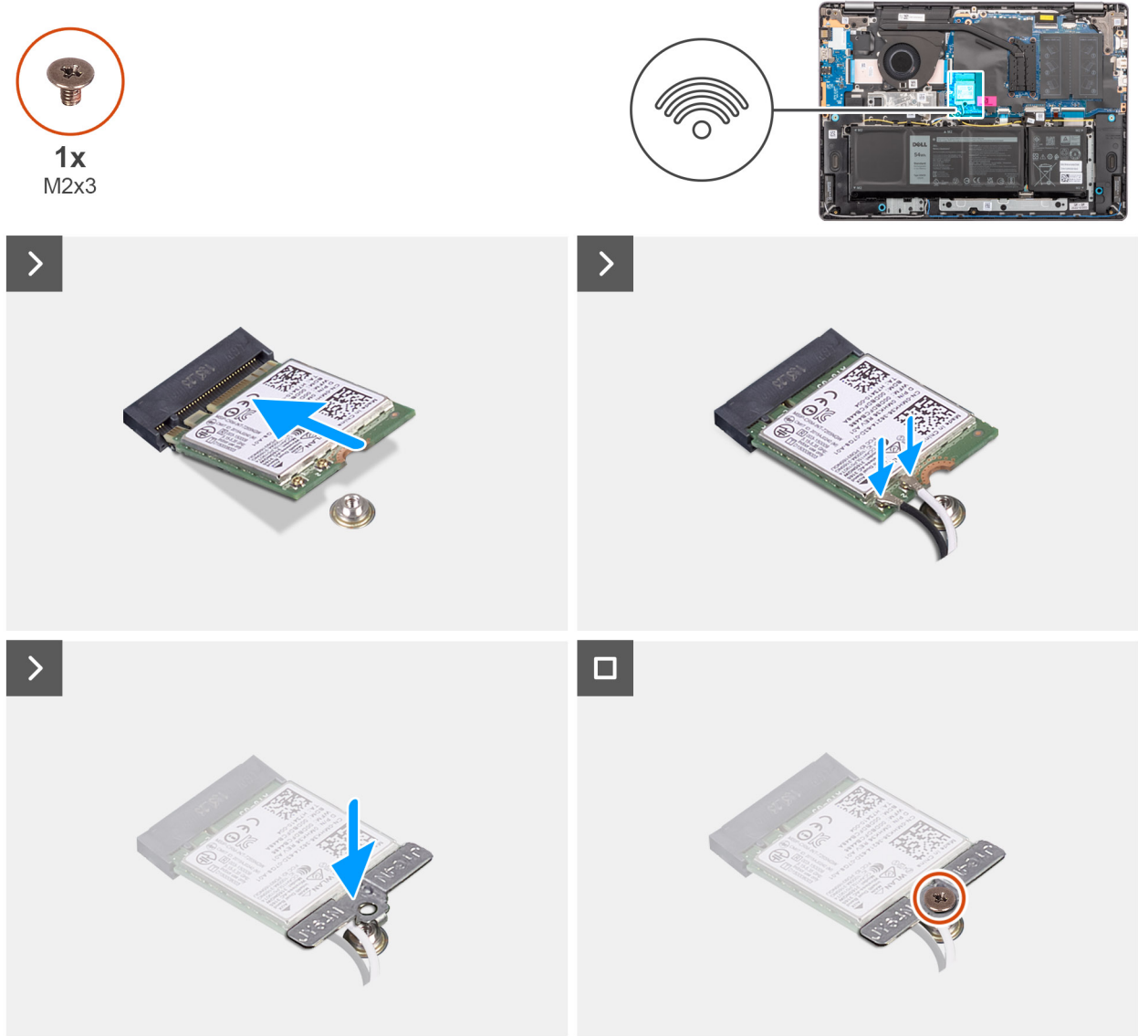
Figure 23. Installing the wireless card
