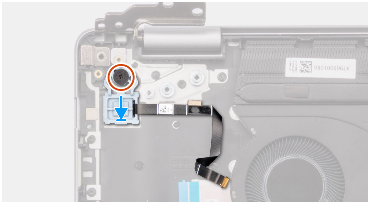
Figure 45. Installing the power button with optional fingerprint reader
