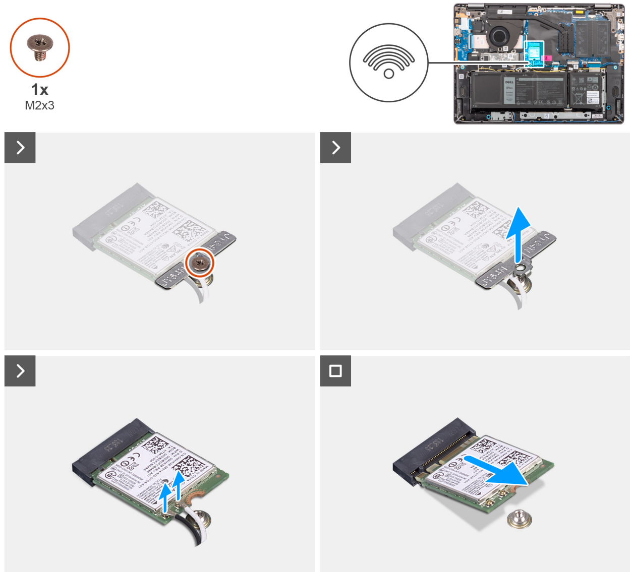
Figure 22. Removing the wireless card
