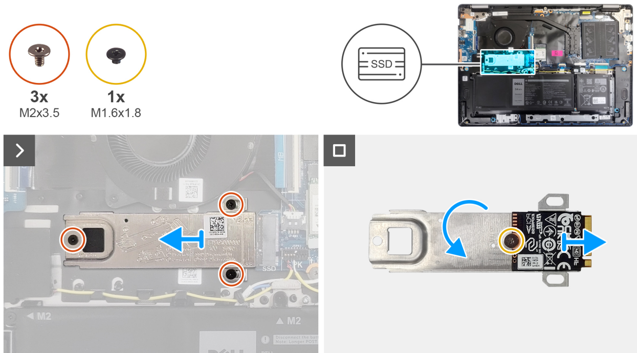
Figure 20. Removing the solid-state drive
