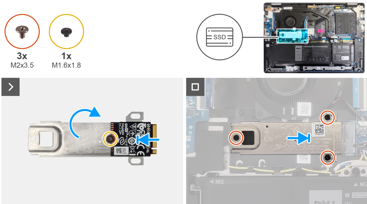
Figure 21. Installing the solid-state drive
