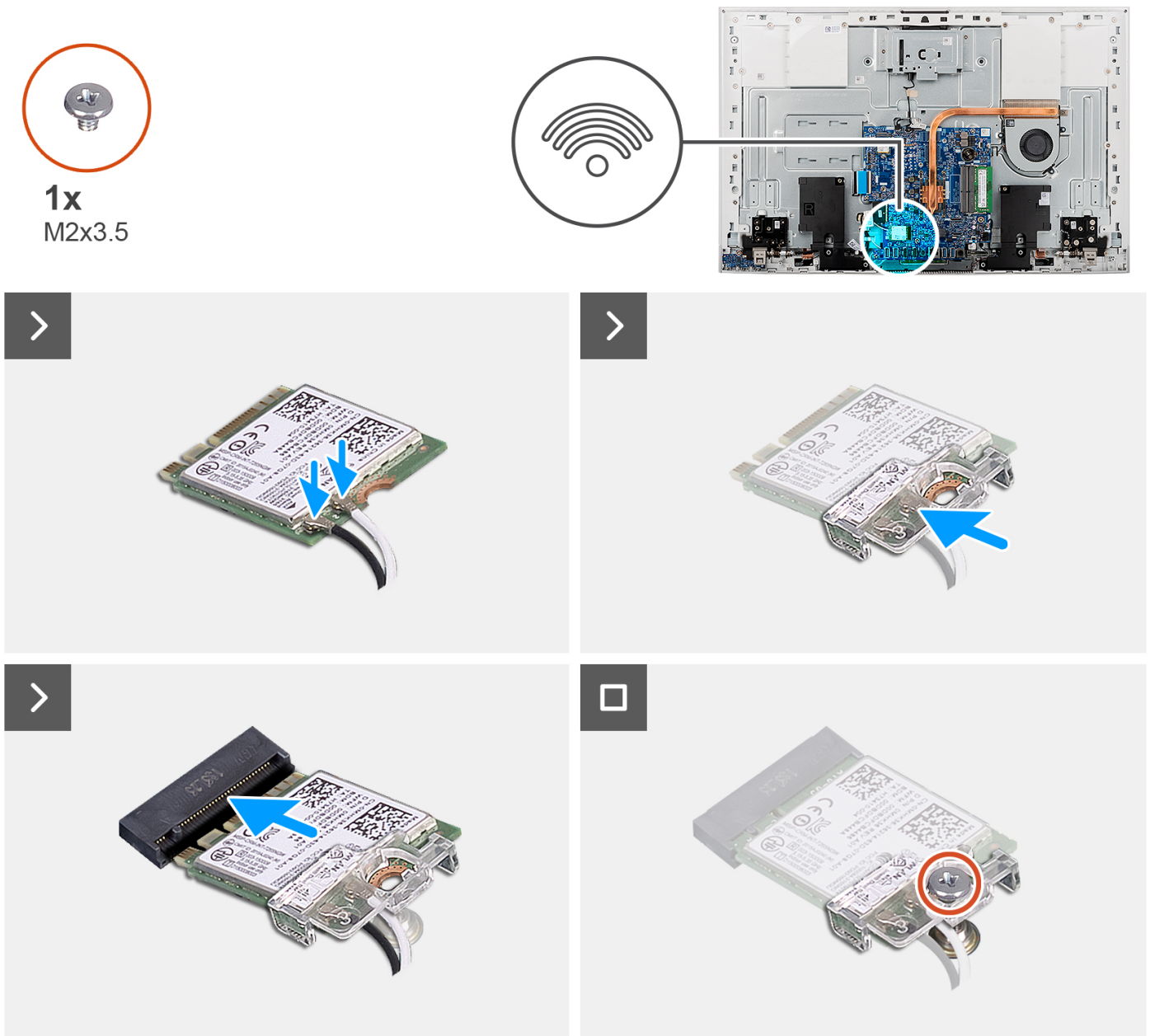
Figure 33. Installing the wireless card
