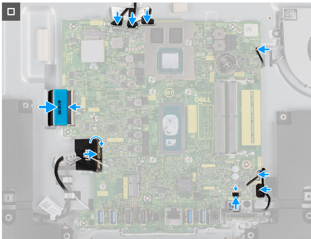
Figure 55. Installing the system board
