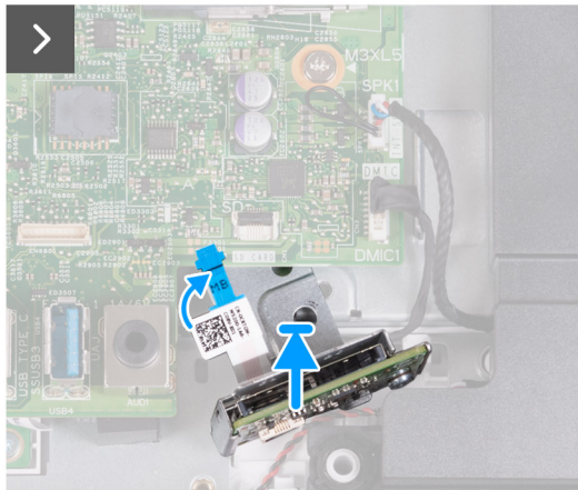
Figure 47. Installing the media-card reader
