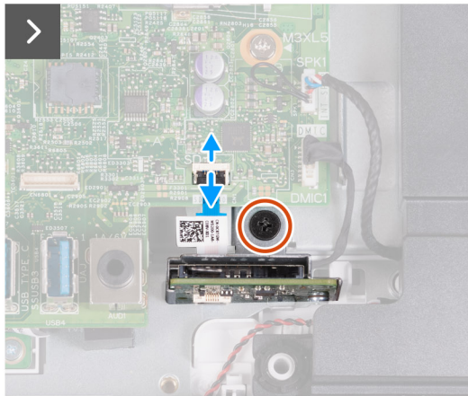
Figure 46. Removing the media-card reader
