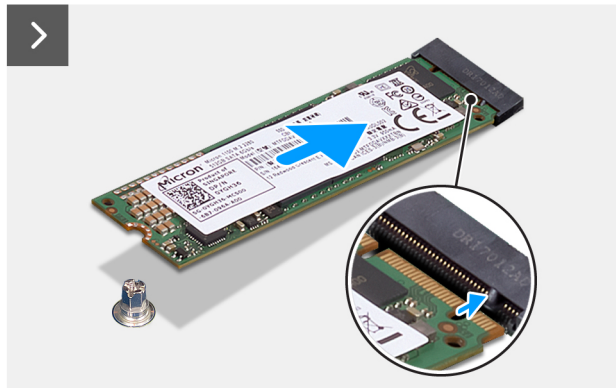
Figure 25. Installing the M.2 2280 solid state drive in slot 0
