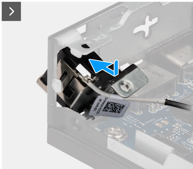
Figure 68. Installing the antenna module (white cable)
