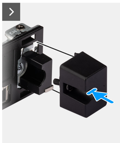
Figure 68. Installing the antenna module (white cable)
