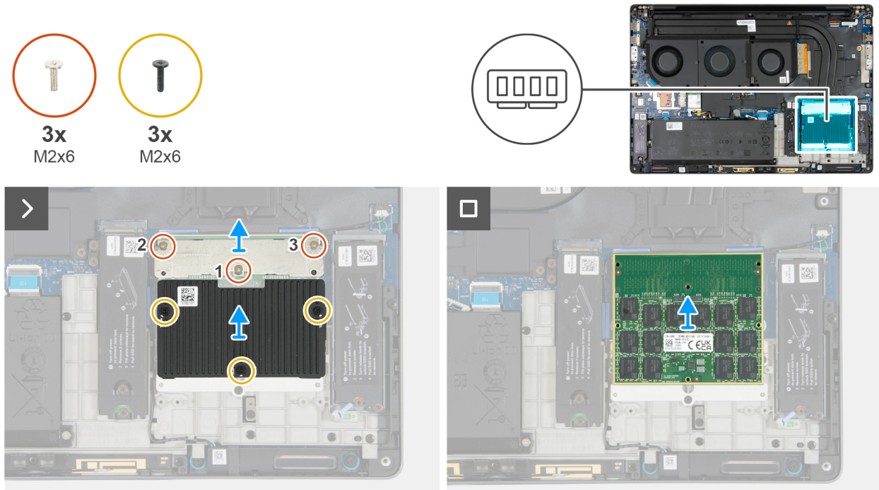
Figure 32. Removing the CAMM module (dual-channel)
