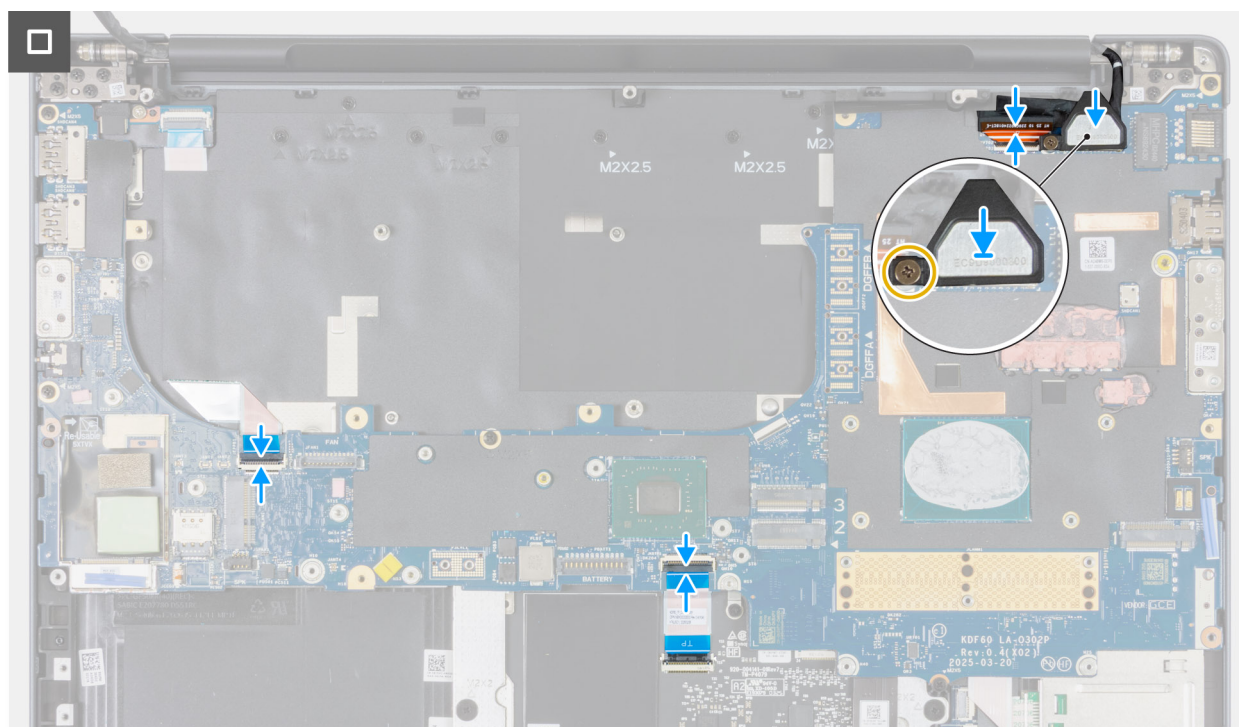
Figure 114. Installing the system board
