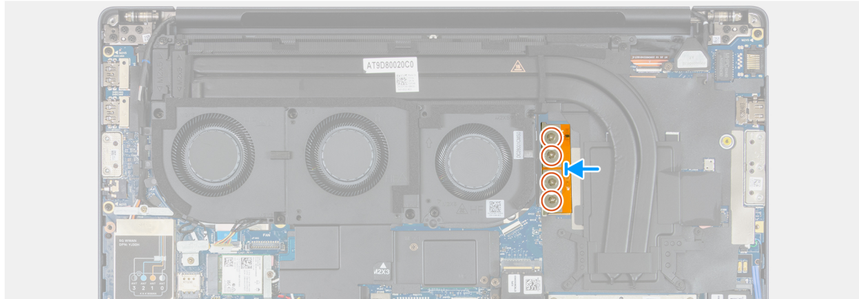
Figure 56. Installing the integrated FPC beam connector
