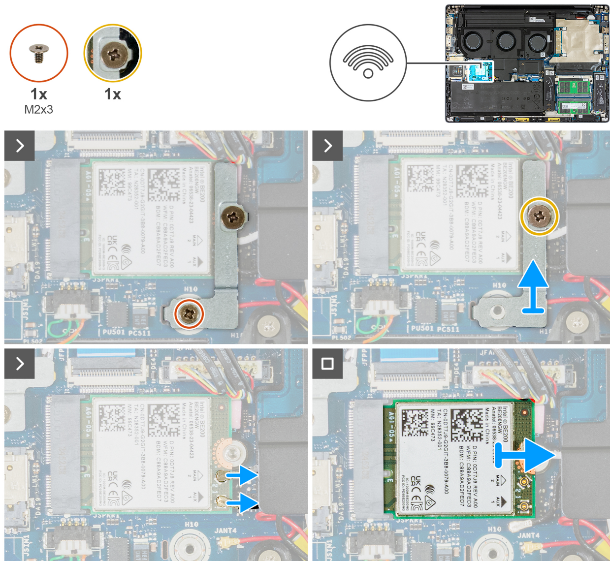
Figure 46. Removing the WLAN card
