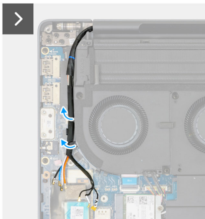
Figure 63. Removing the display assembly
