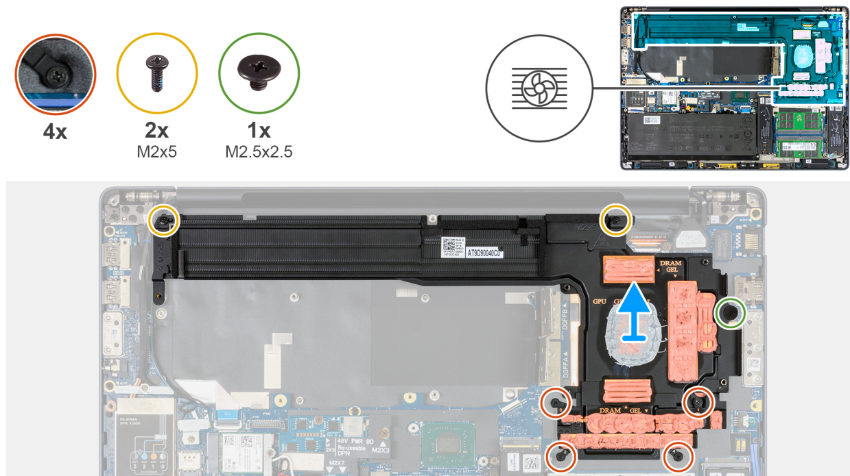
Figure 75. Removing the heat sink for computers shipped with discrete graphics
