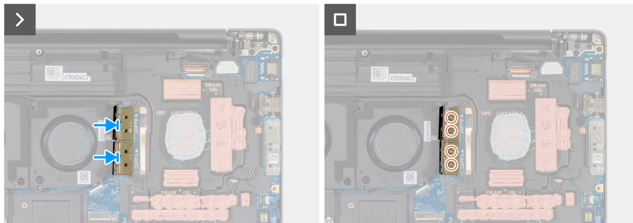
Figure 58. Installing the discrete FPC beam connector
