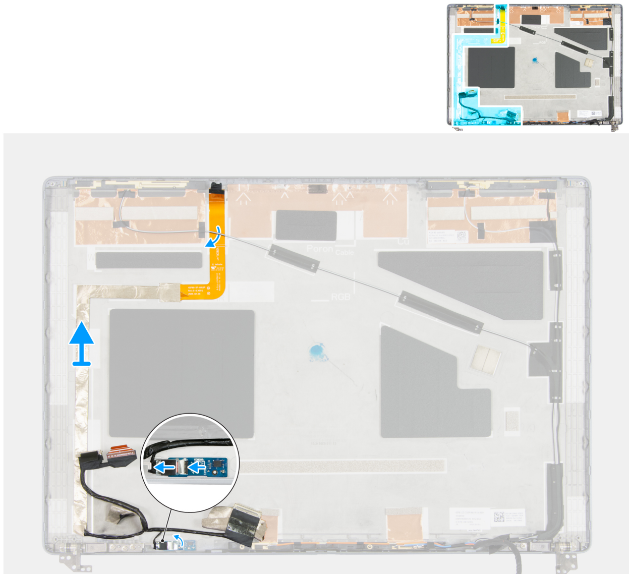
Figure 104. Removing the display cable
