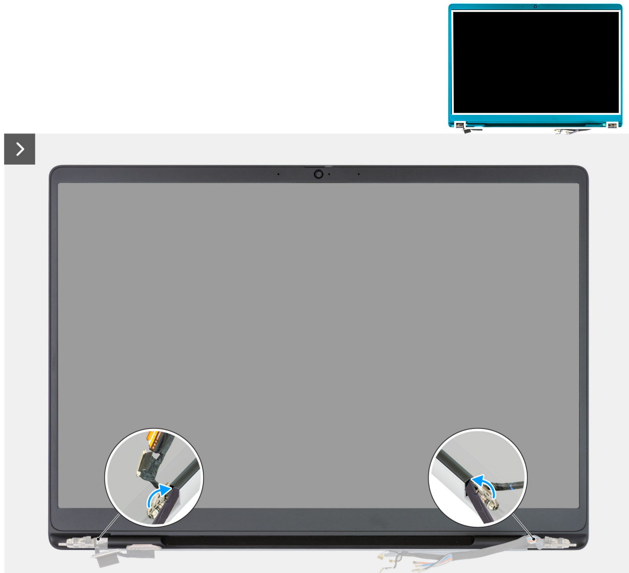
Figure 83. Removing the display bezel
