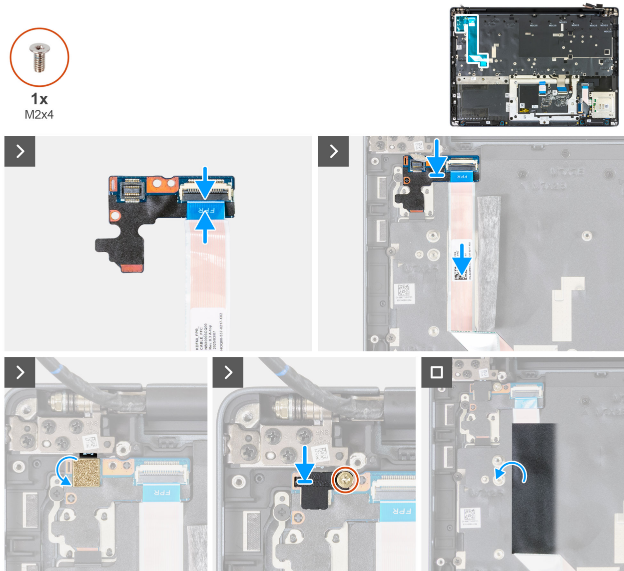
Figure 126. Installing the power button board
