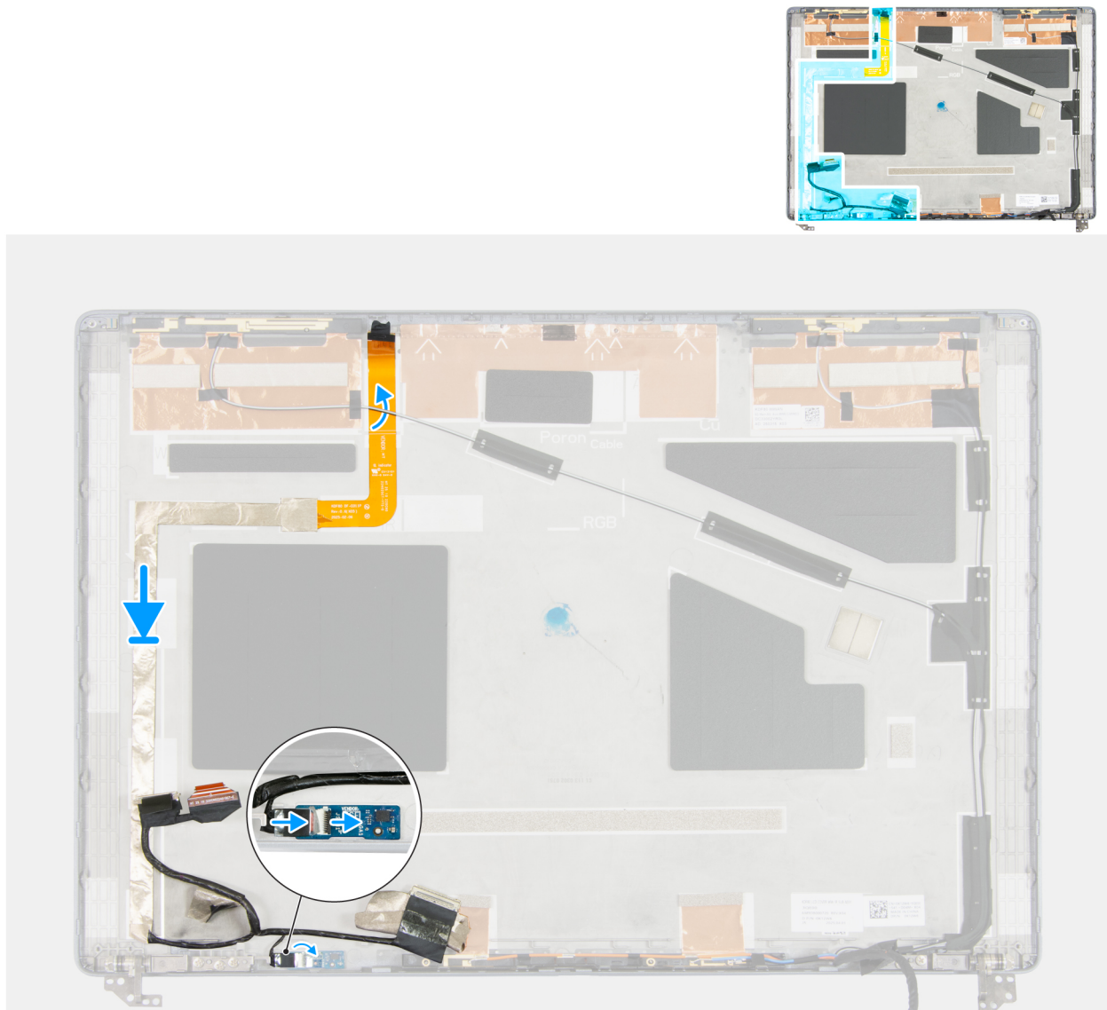
Figure 105. Installing the display cable
