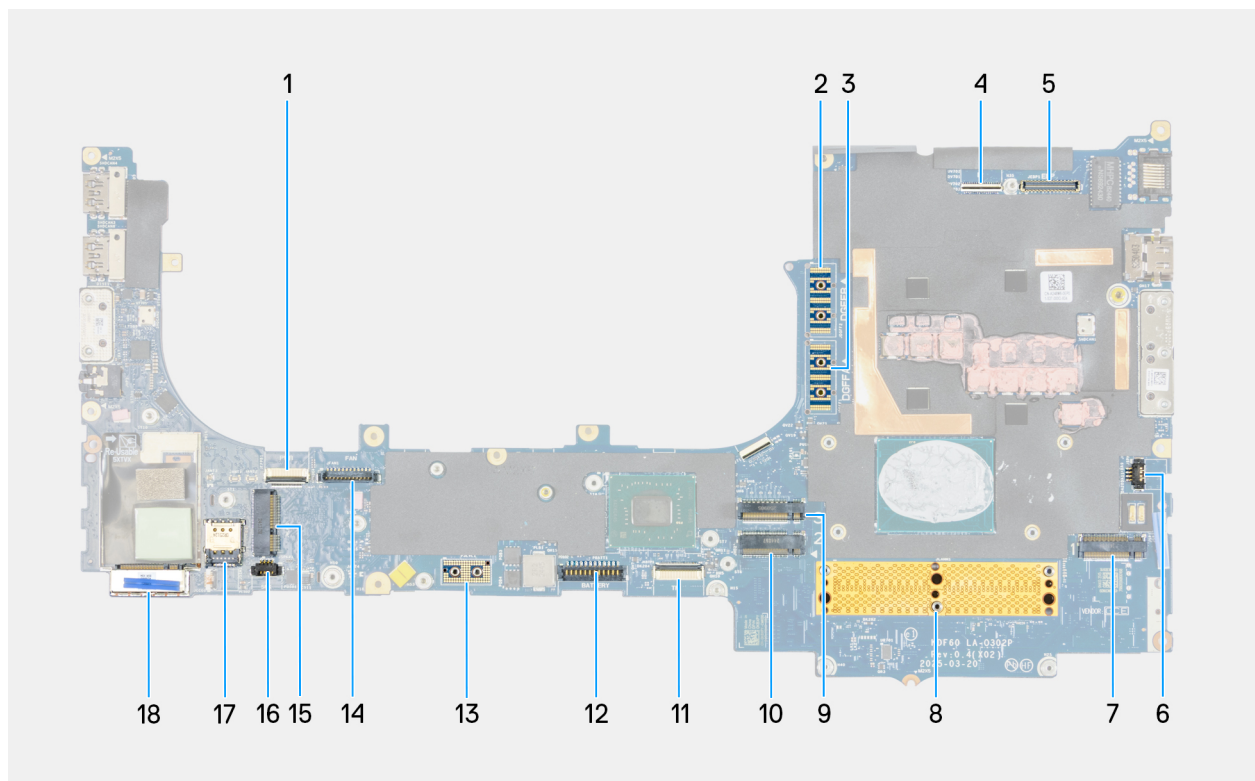
Figure 108. System-board components
