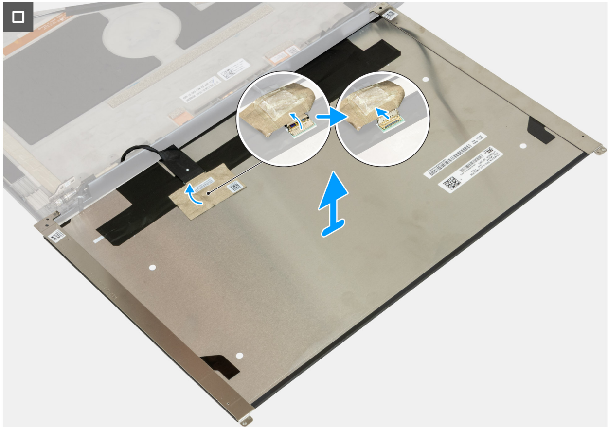
Figure 96. Removing the display panel for non-touchscreen displays
