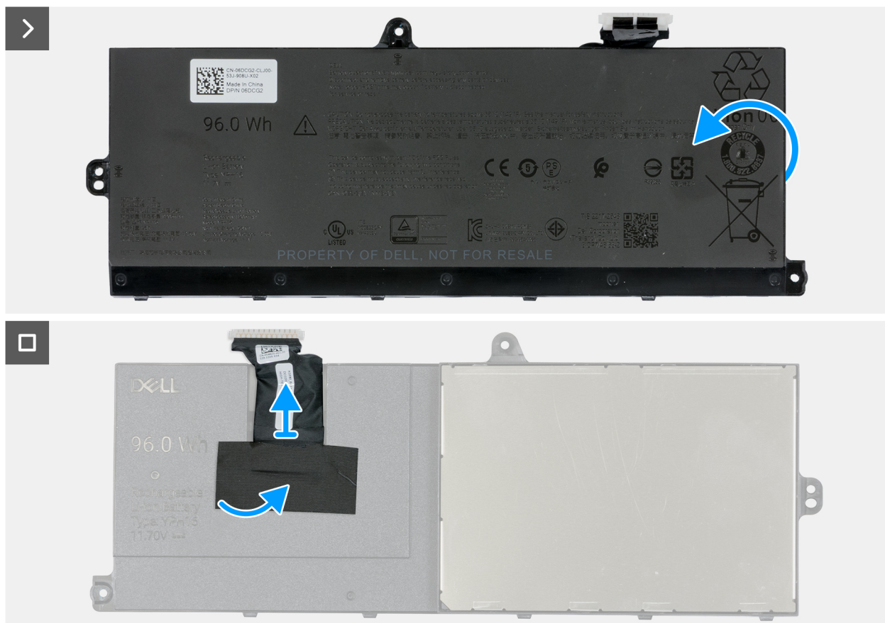
Figure 43. Removing the battery cable from the battery
