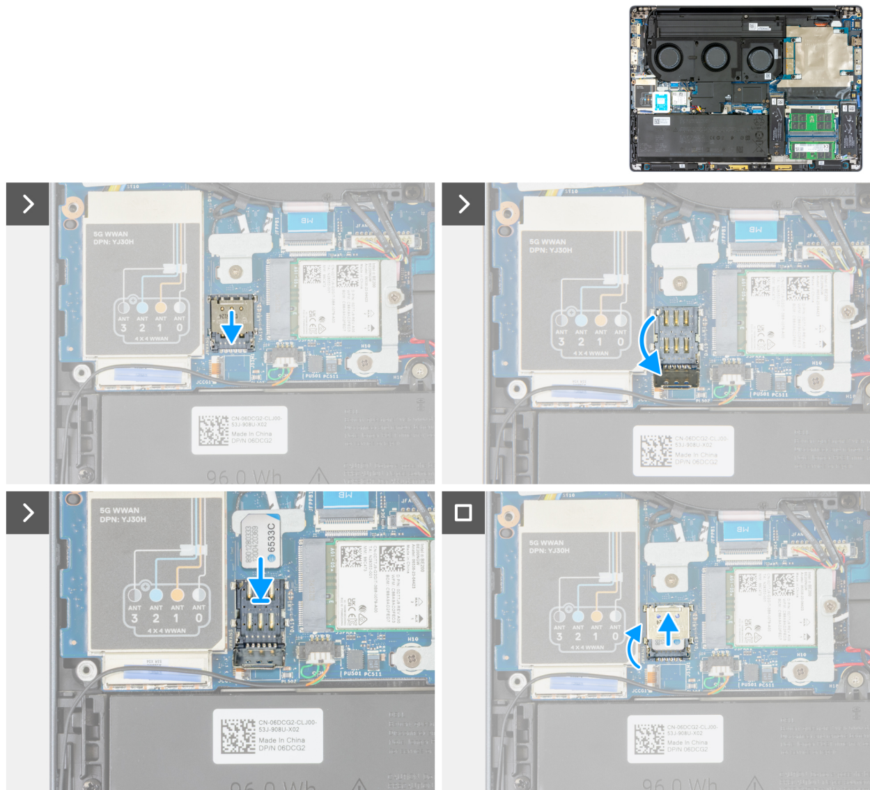
Figure 49. Installing the SIM card
