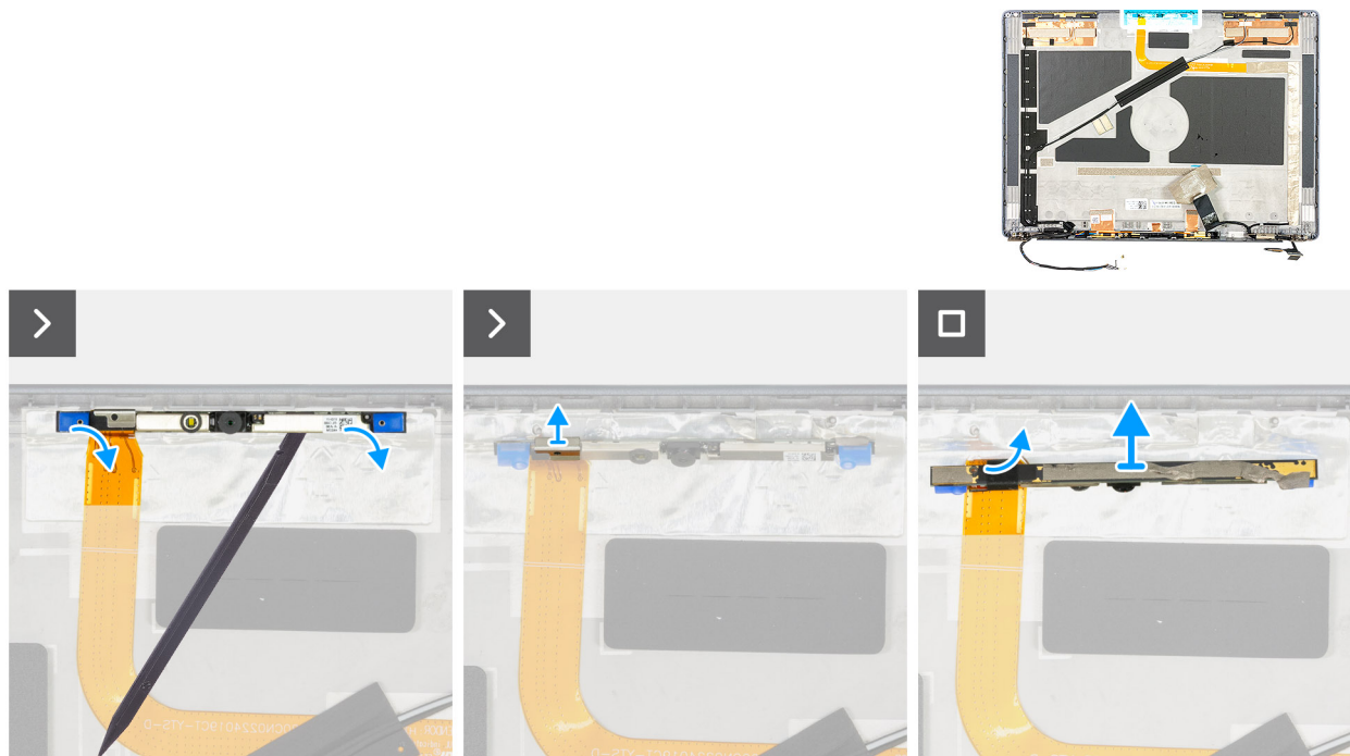
Figure 101. Removing the camera module
