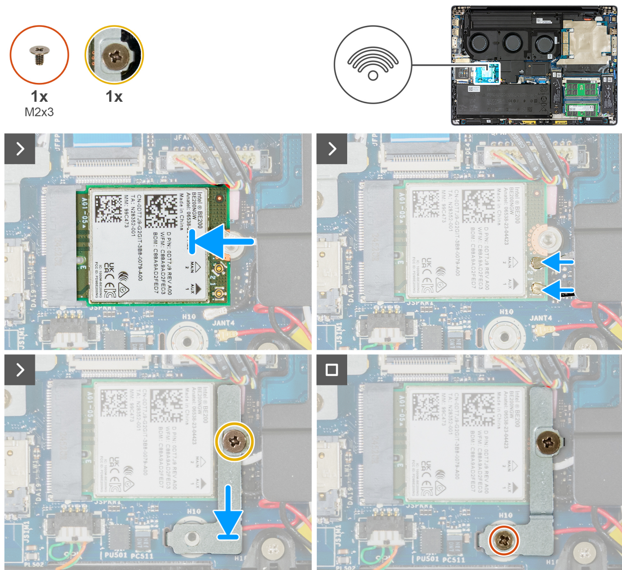
Figure 47. Installing the WLAN card
