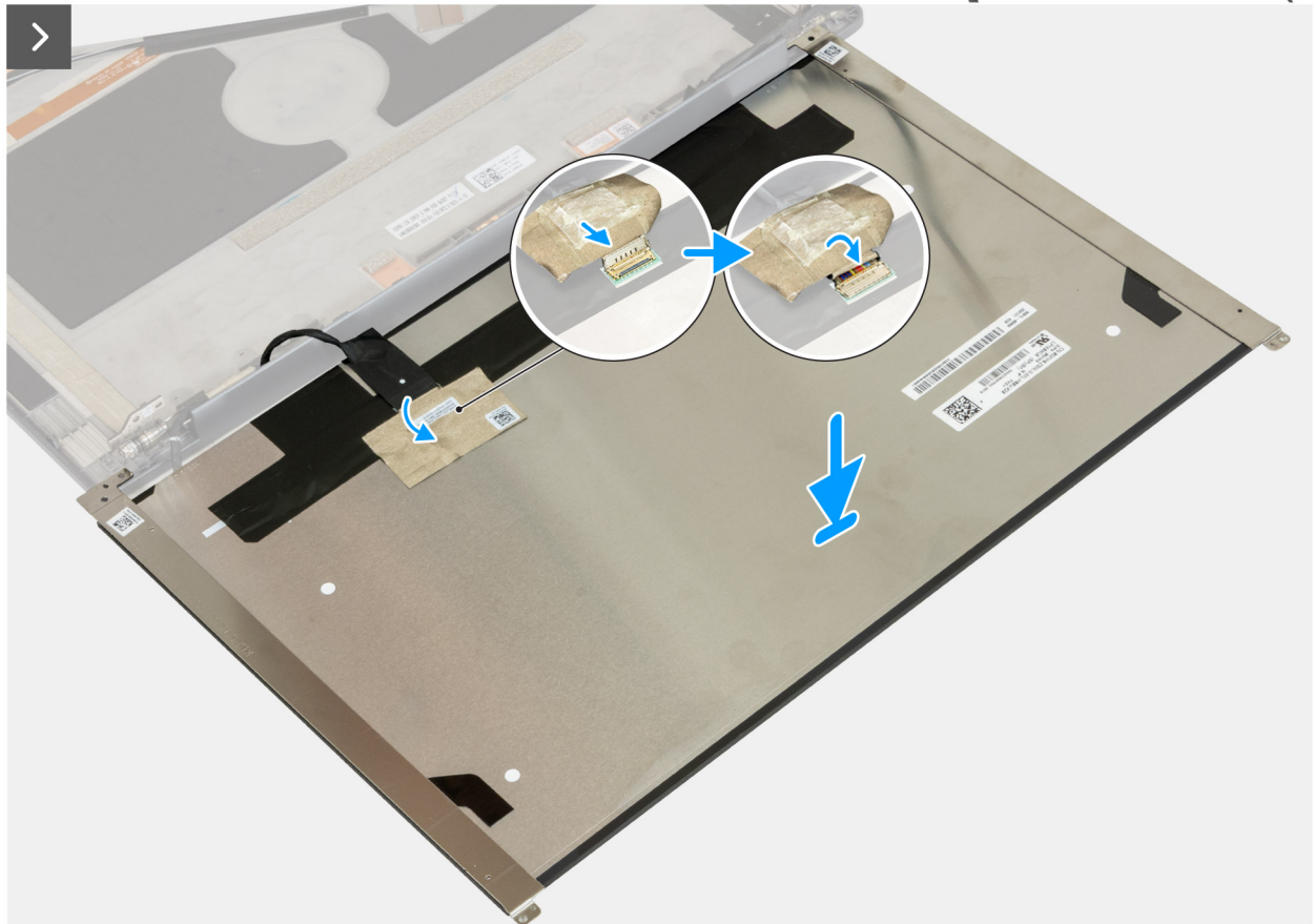
Figure 97. Installing the display panel for non-touchscreen displays
