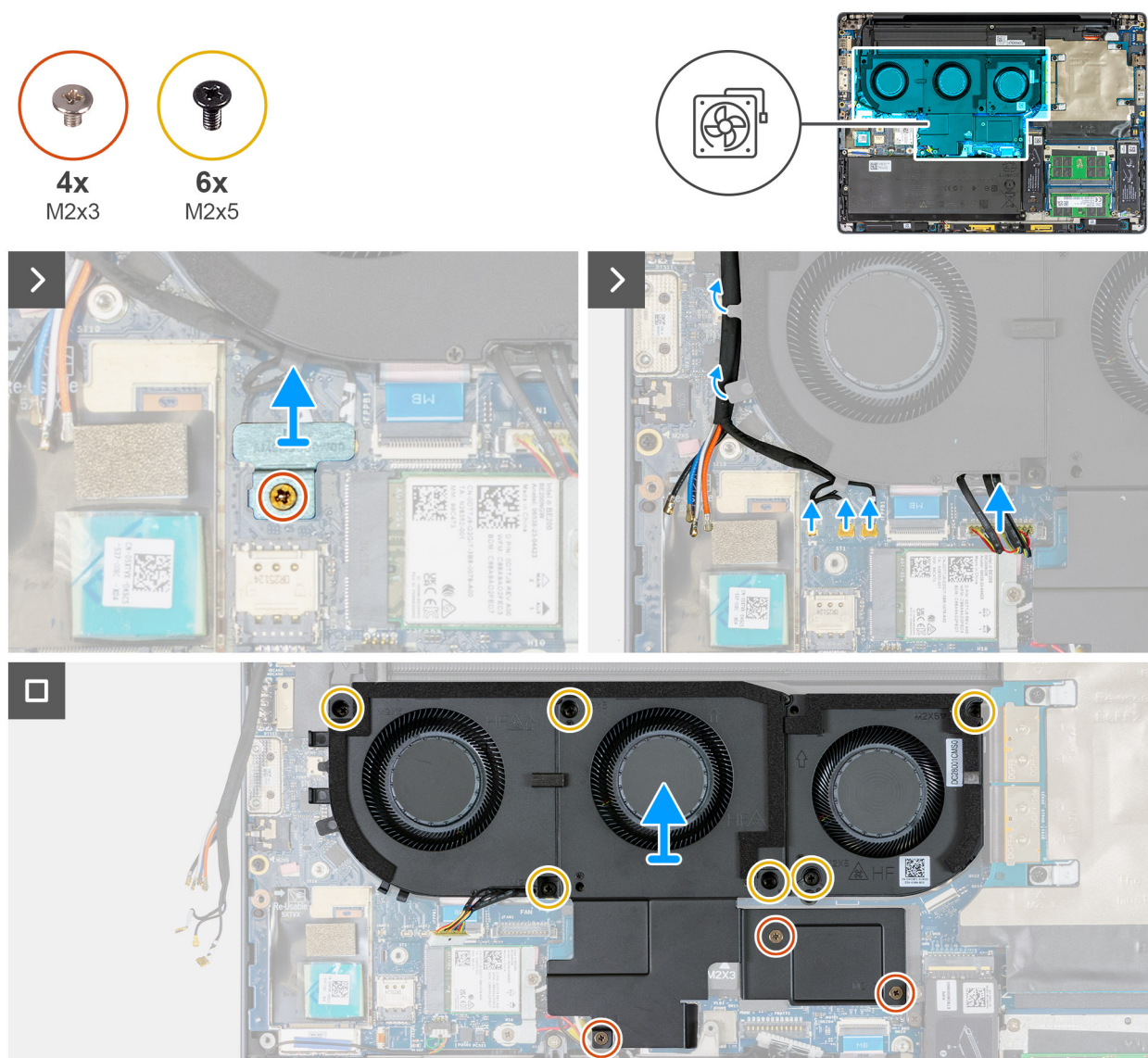
Figure 61. Removing the fan assembly
