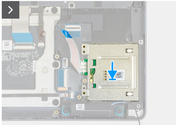
Figure 122. Installing the smart card reader
