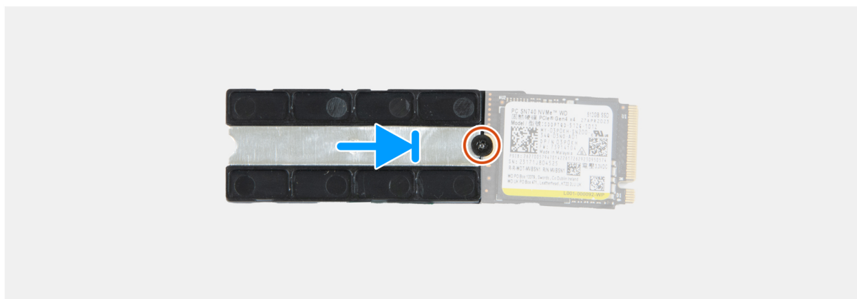
Figure 41. Installing the M.2 2230 SSD
