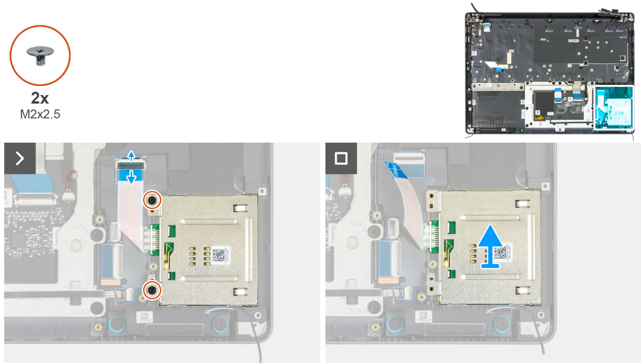
Figure 121. Removing the smart card reader
