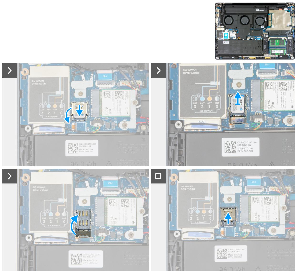
Figure 48. Removing the SIM card
