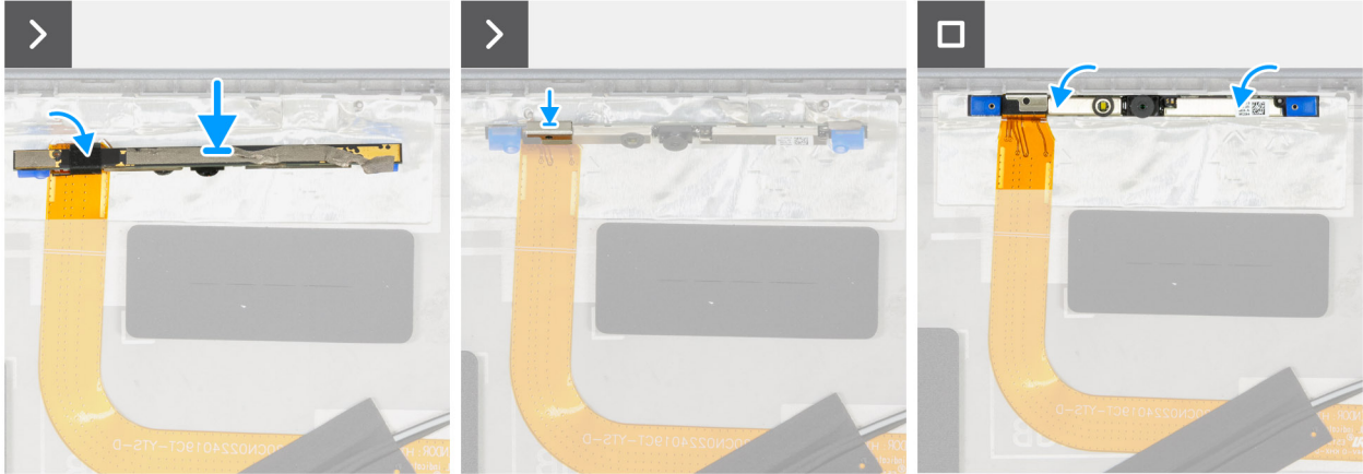
Figure 102. Installing the camera module
