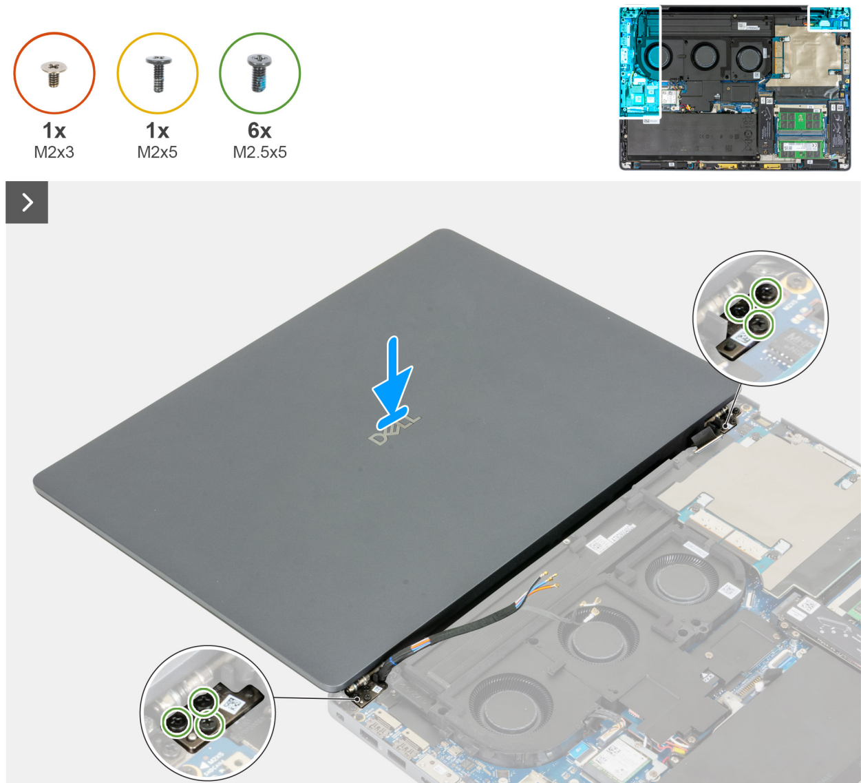
Figure 65. Installing the display assembly
