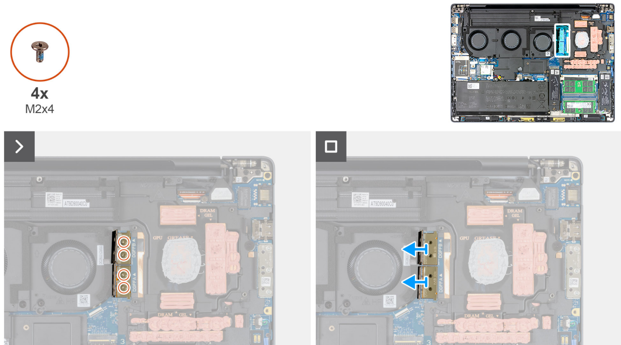
Figure 57. Removing the discrete FPC beam connector
