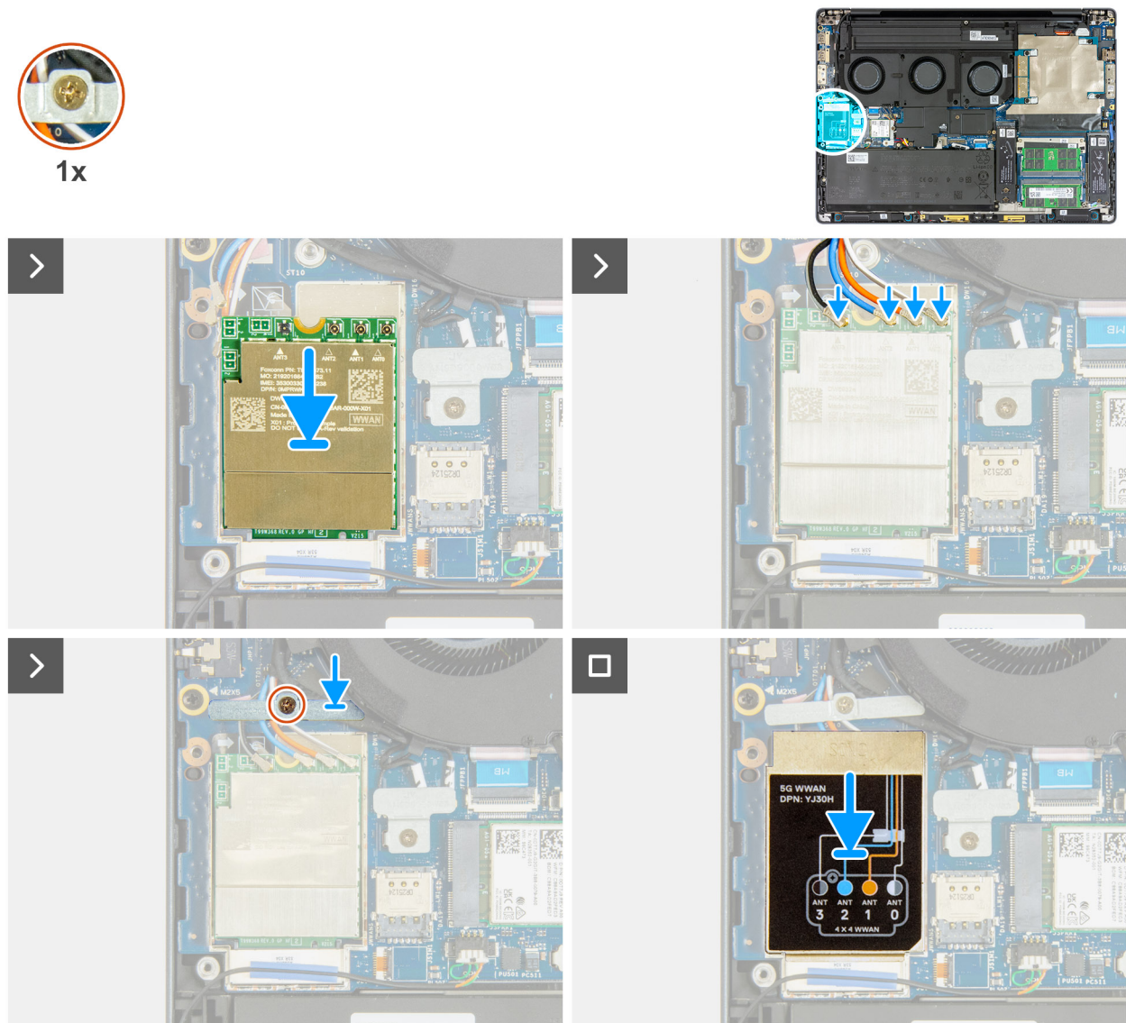
Figure 51. Installing the WWAN card
