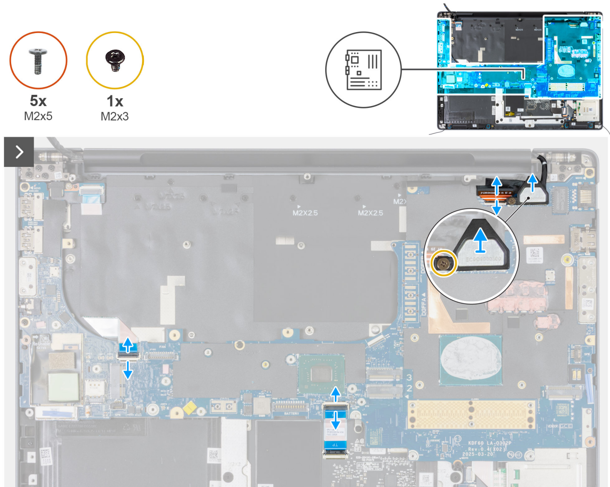
Figure 109. Removing the system board
