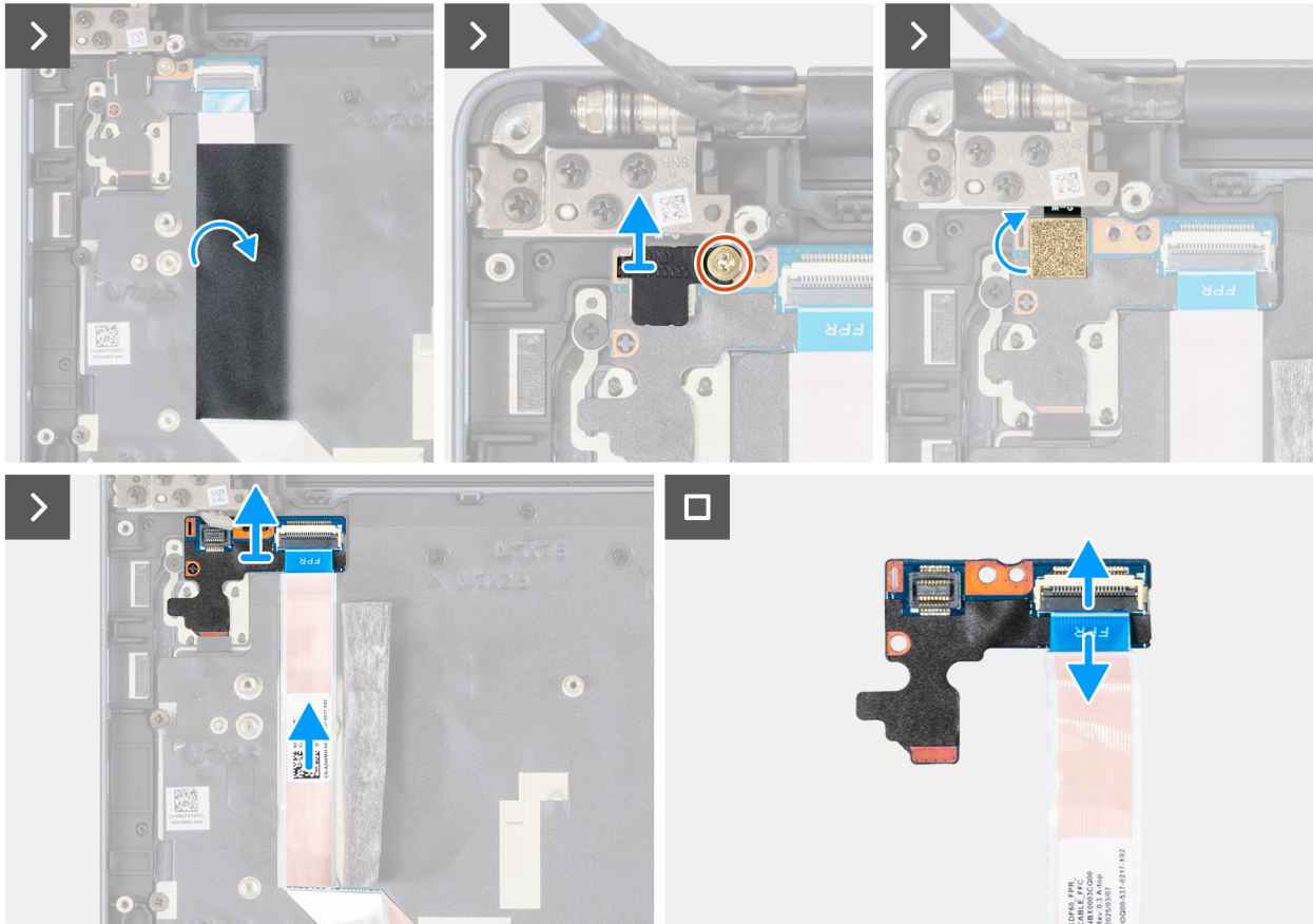
Figure 125. Removing the power button board
