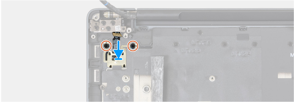
Figure 128. Installing the power button
