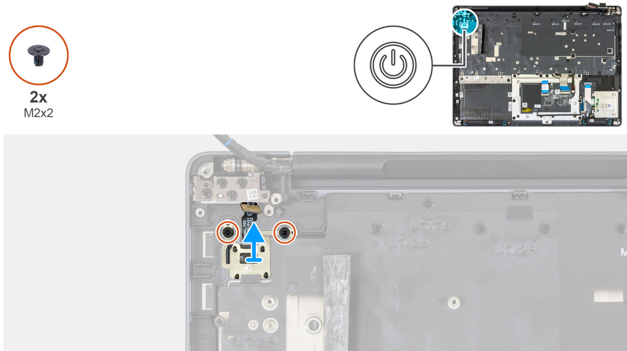
Figure 127. Removing the power button
