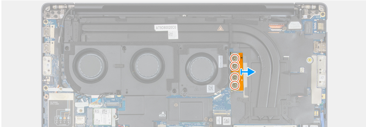
Figure 55. Removing the integrated FPC beam connector
