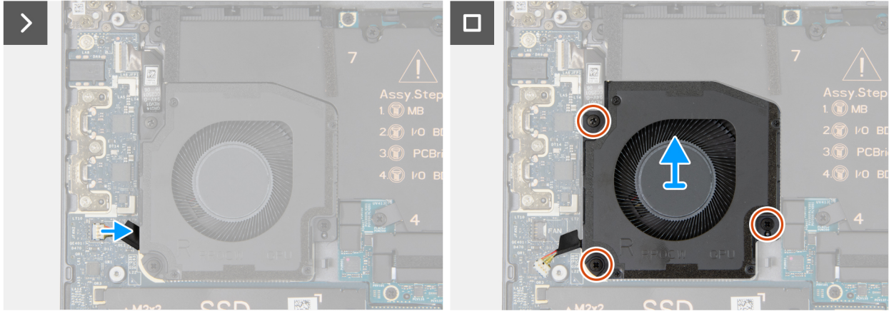
Figure 29. Removing the right fan
