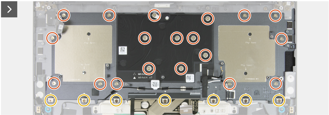
Figure 71. Removing the keyboard
