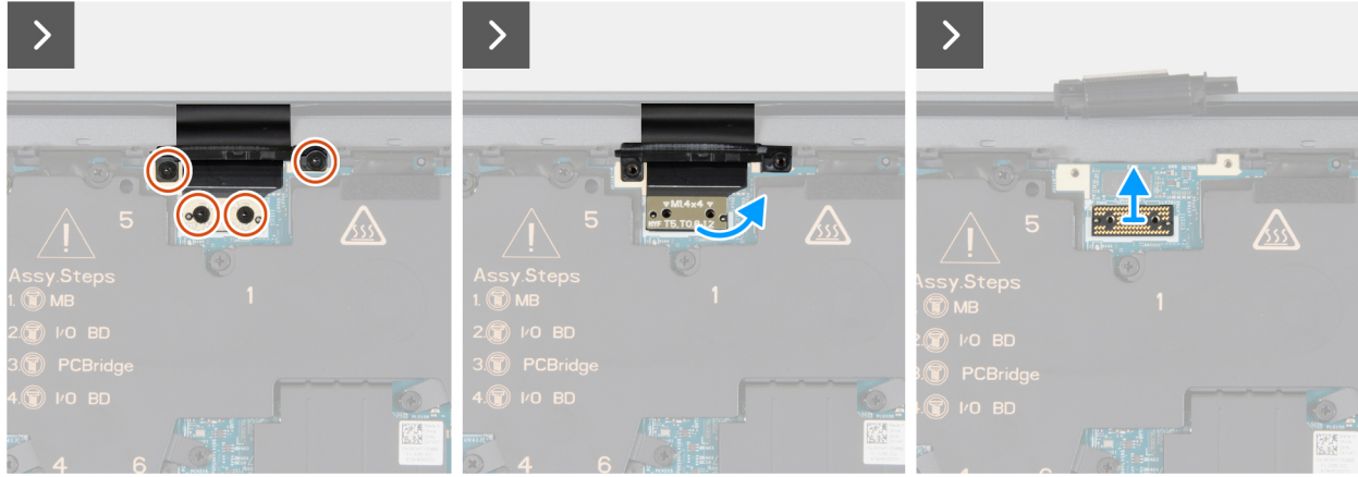
Figure 31. Removing the display assembly
