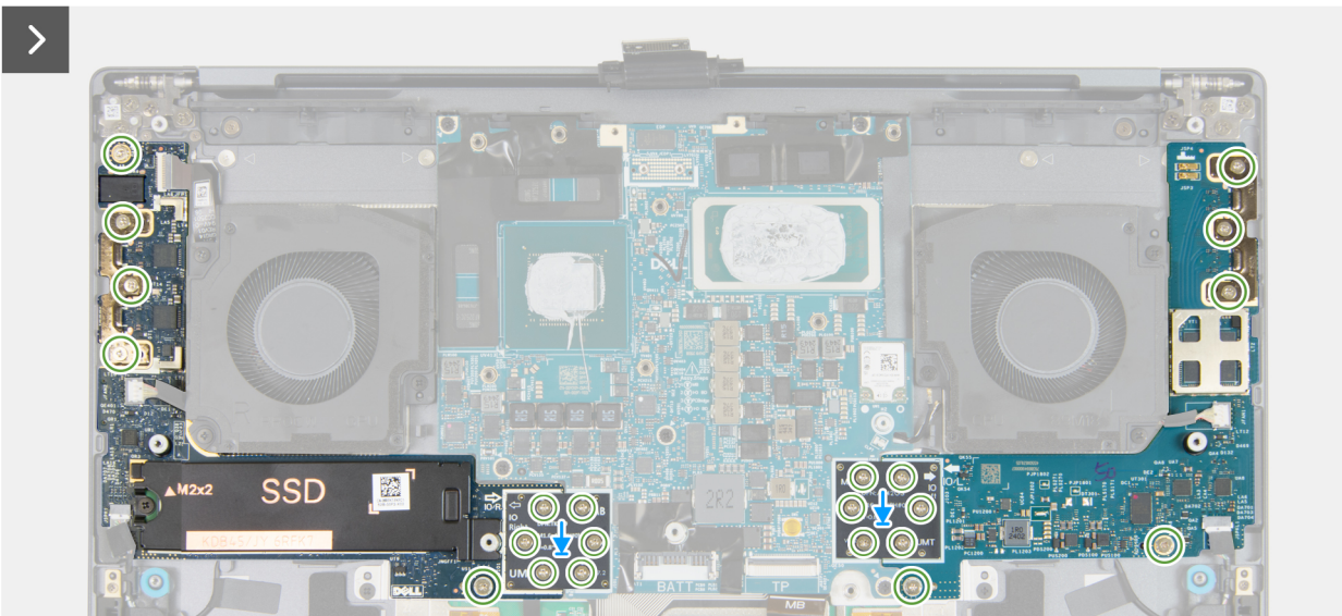
Figure 63. Installing the system board (discrete graphics)
