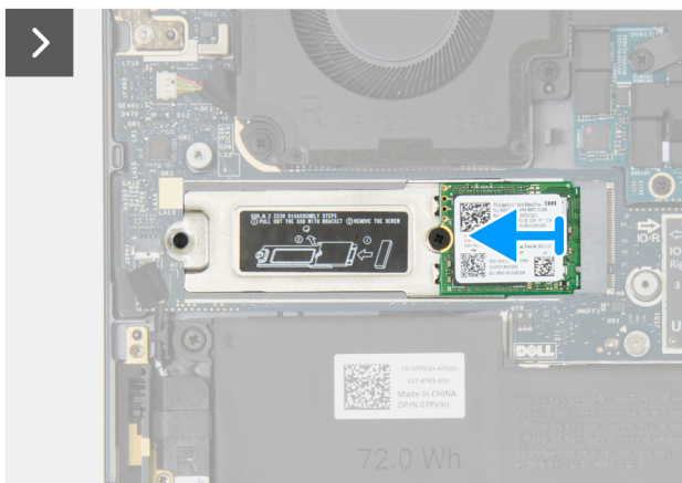
Figure 25. Removing the M.2 2230 solid state drive
