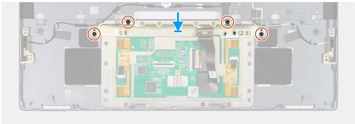
Figure 80. Replacing the touchpad bracket
