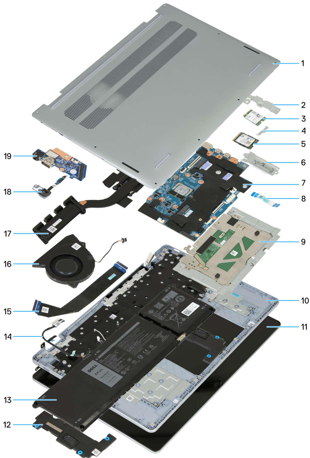
Figure 8. Image: Major components of Dell 16 Plus DB16250
