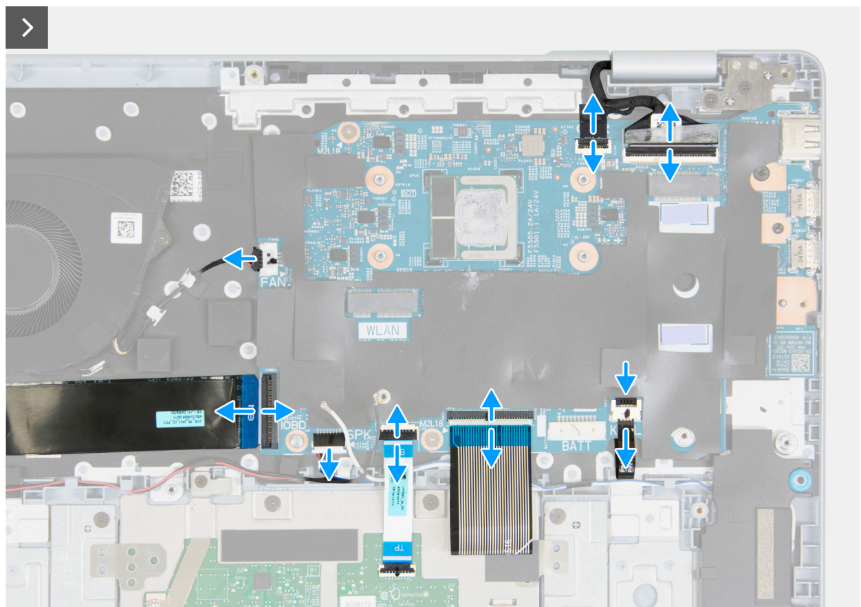
Figure 42. Removing the system board
