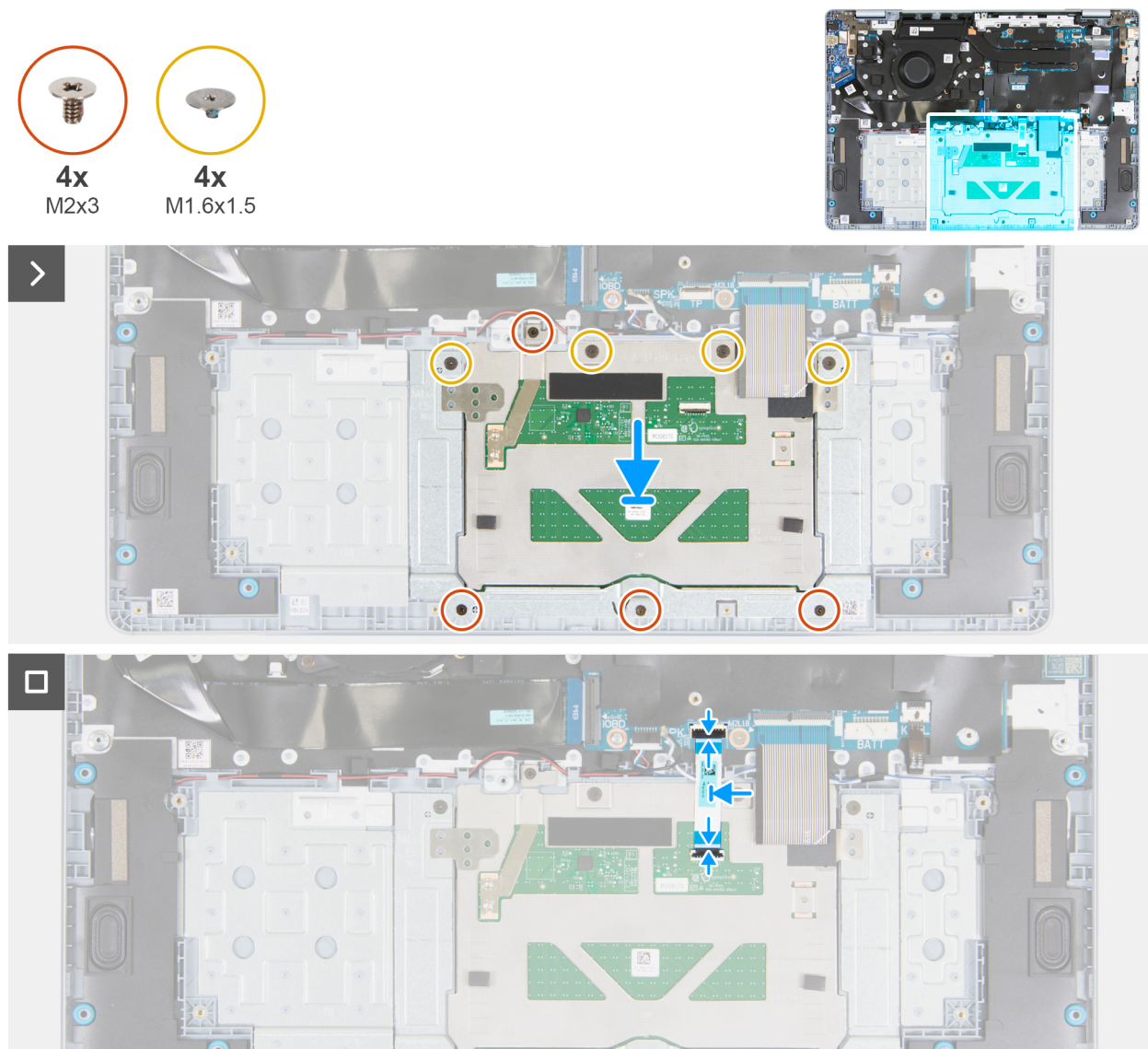
Figure 53. Installing the touchpad
