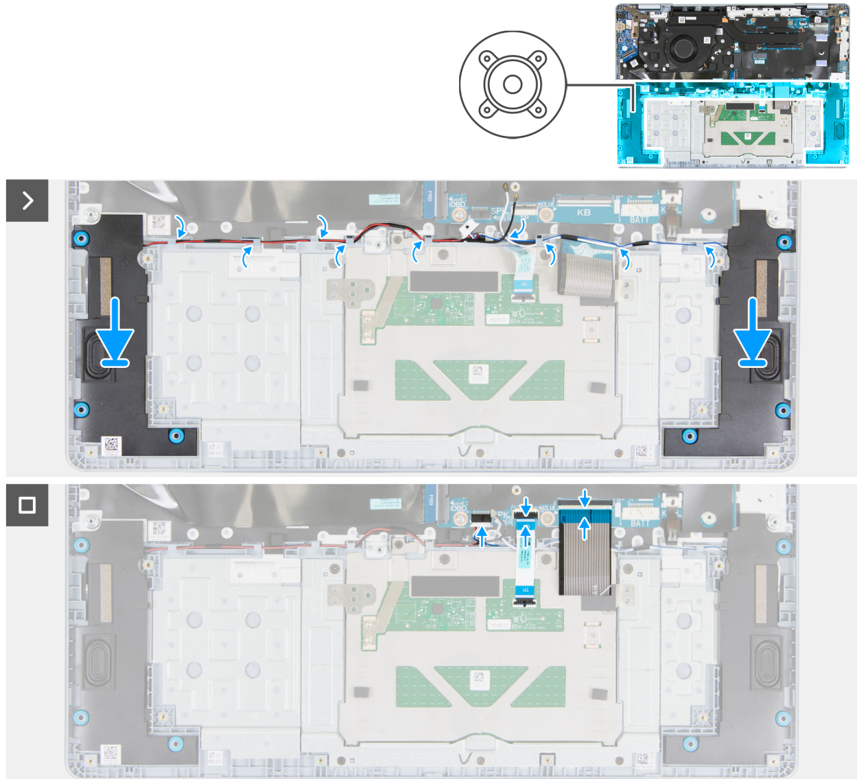
Figure 26. Installing the speaker assembly
