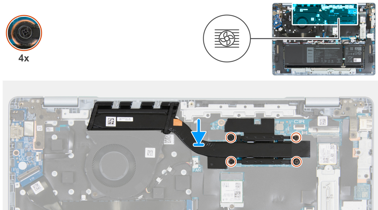
Figure 51. Installing the heat sink
