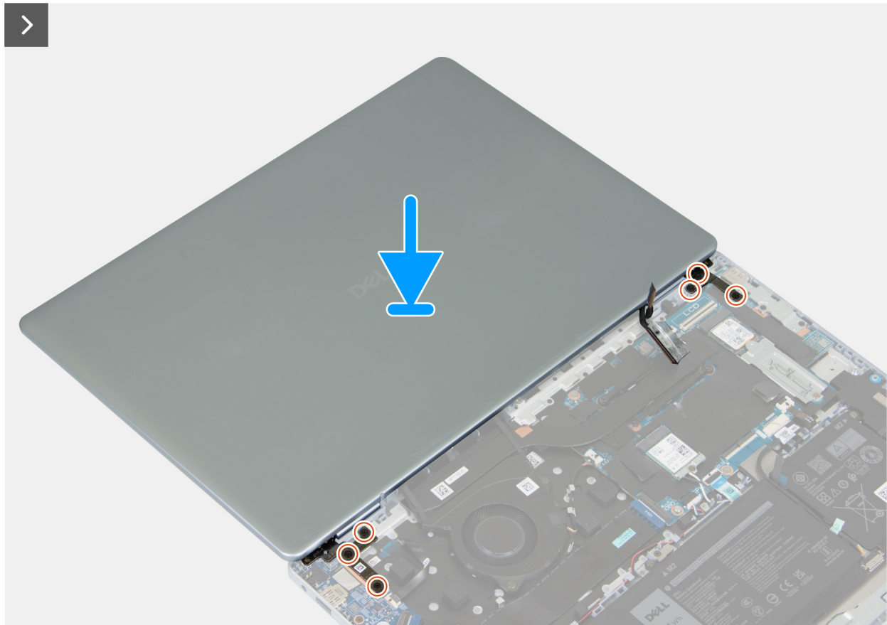
Figure 30. Installing the display assembly 1
