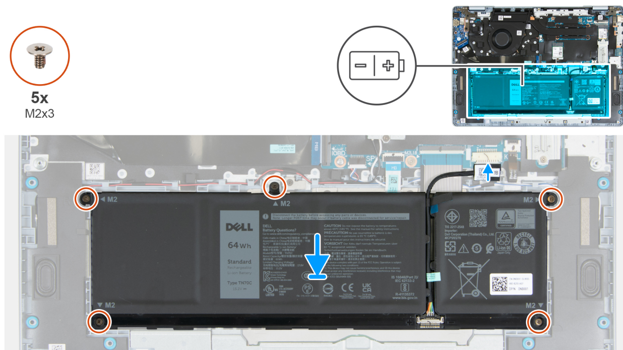
Figure 16. Installing the battery
