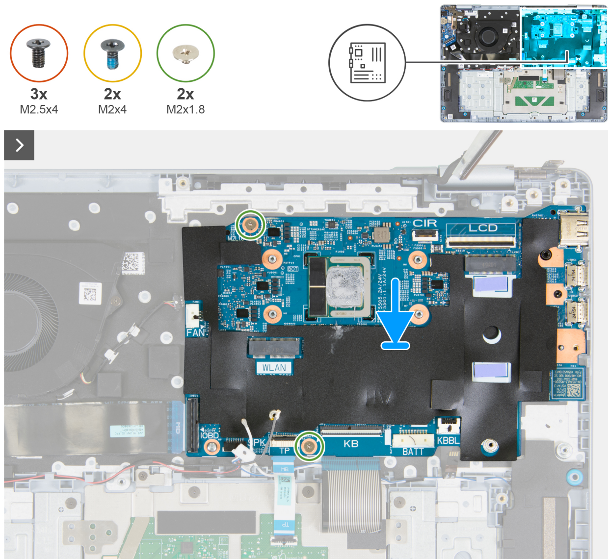
Figure 46. Installing the system board 1
