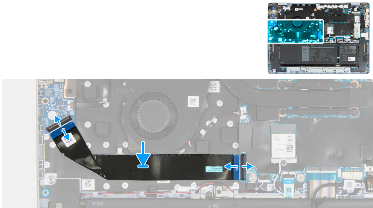
Figure 33. Installing the I/O-board cable
