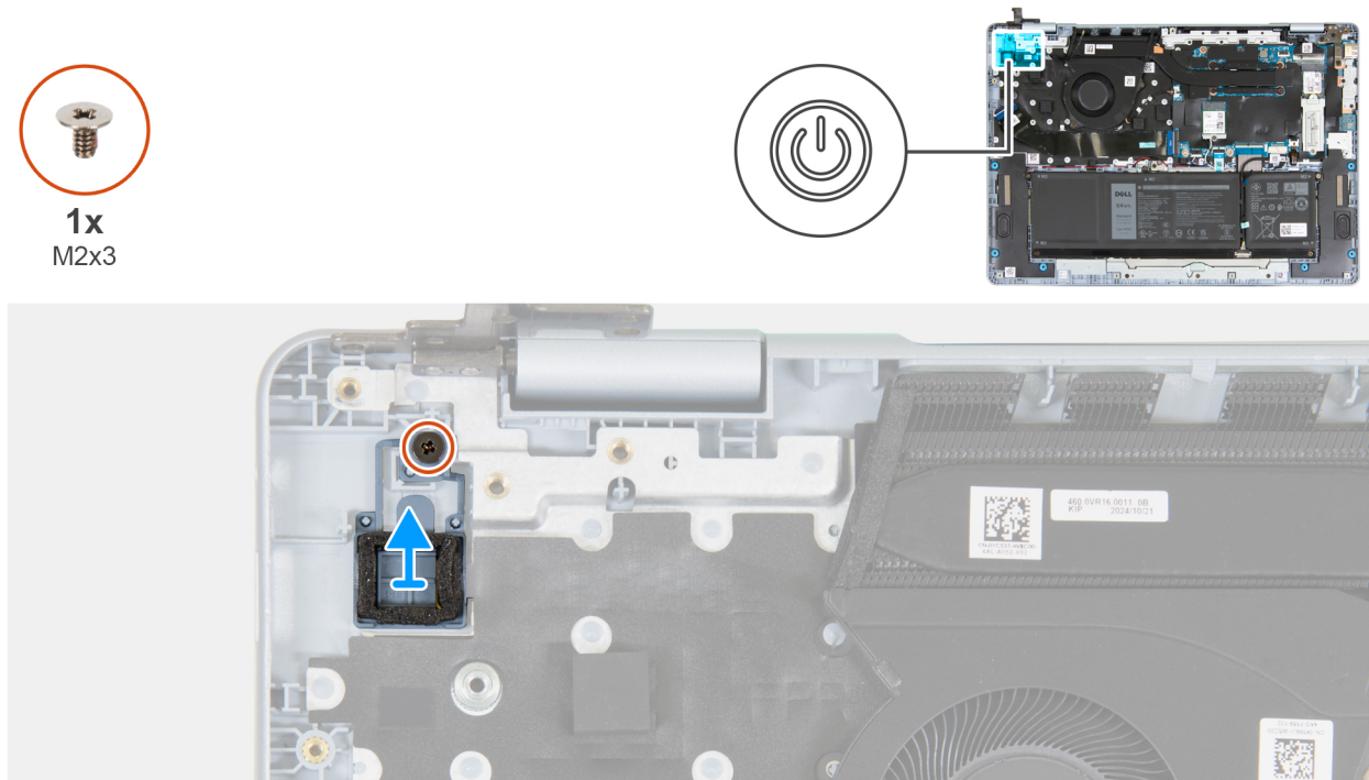
Figure 36. Removing the power button
