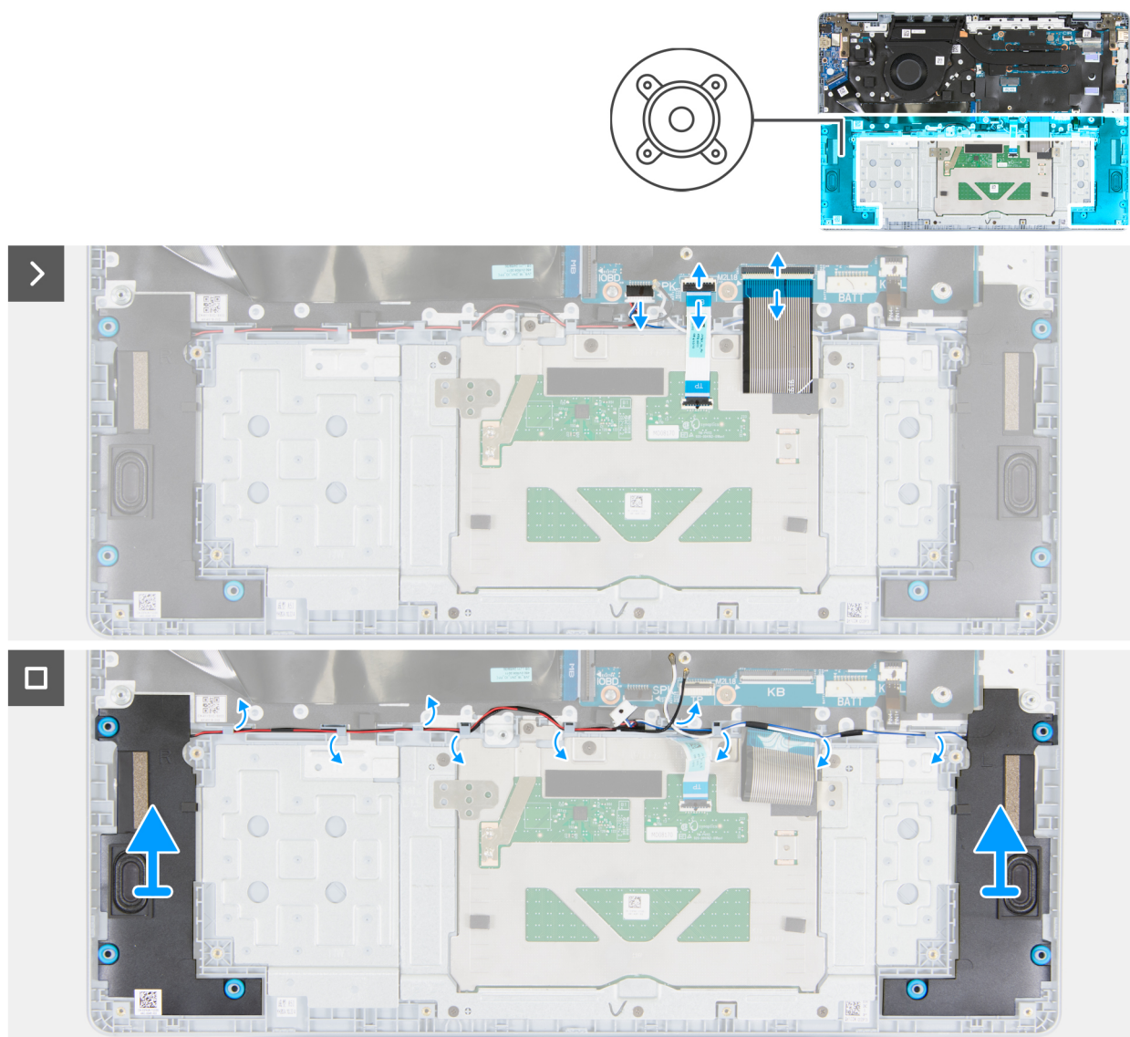
Figure 25. Removing the speaker assembly
