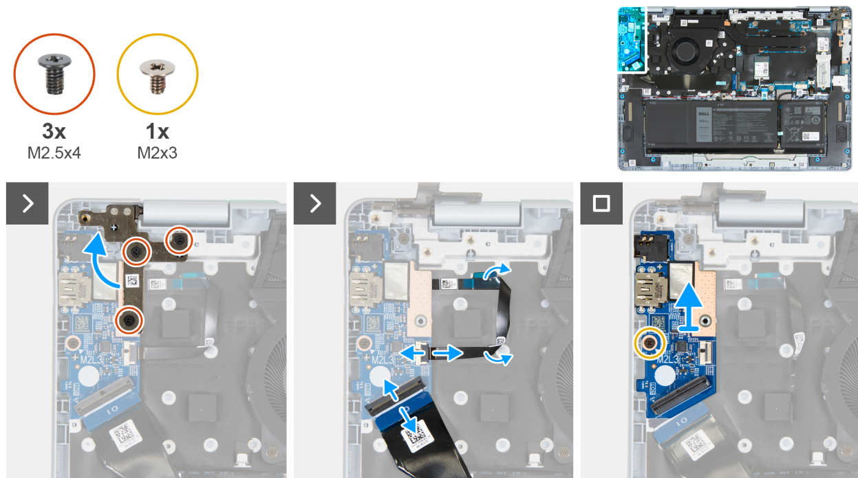
Figure 34. Removing the I/O board
