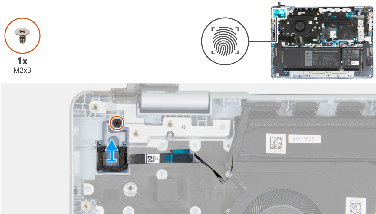
Figure 38. Removing the power button with optional fingerprint reader
