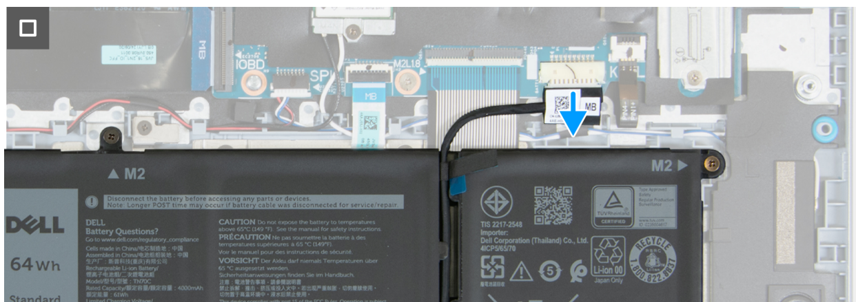
Figure 11. Disconnecting the battery cable
