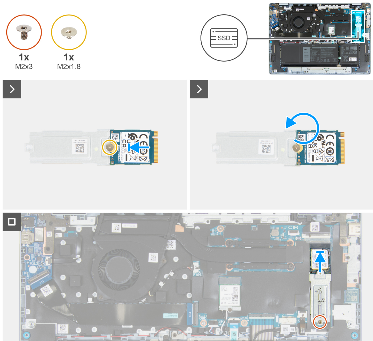
Figure 20. Installing the M.2 2230 solid state drive
