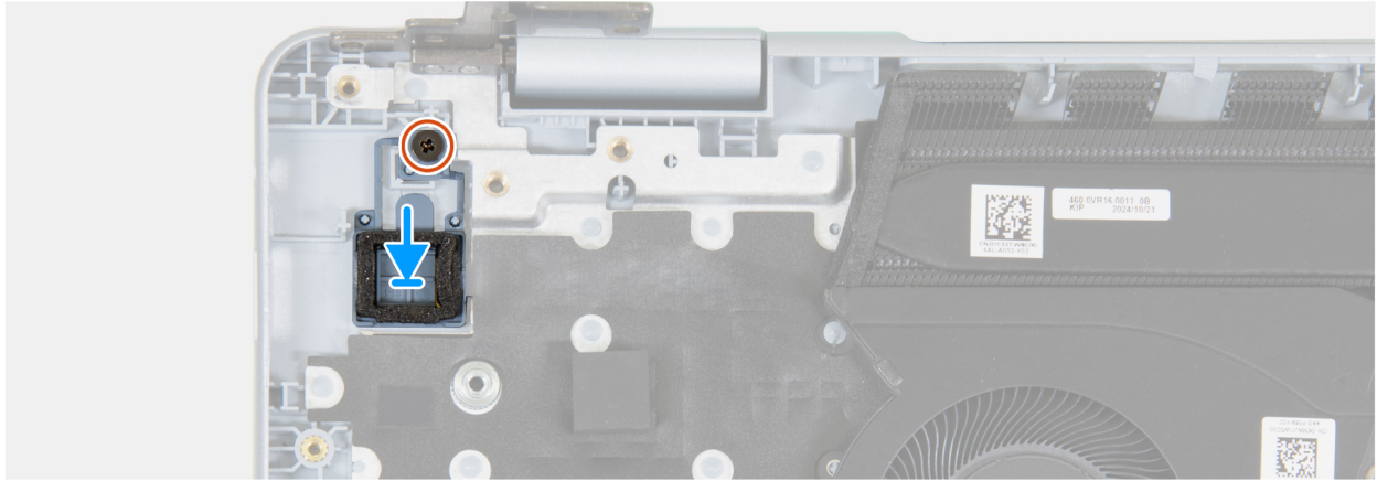
Figure 37. Installing power button
