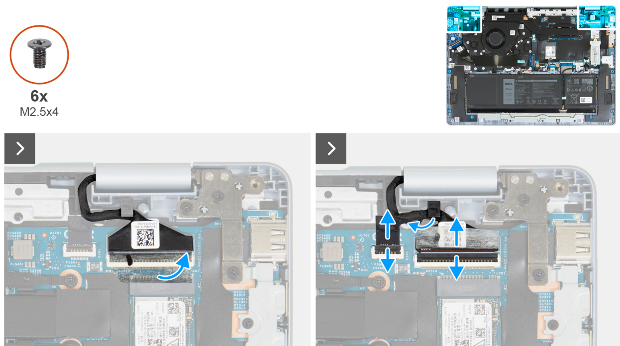
Figure 27. Removing the display assembly 1
