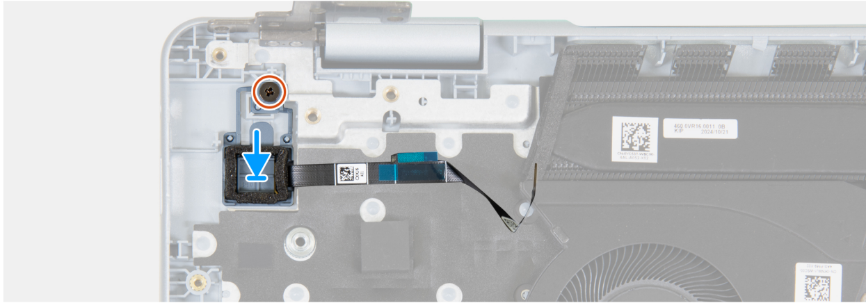
Figure 39. Installing power button with optional fingerprint reader
