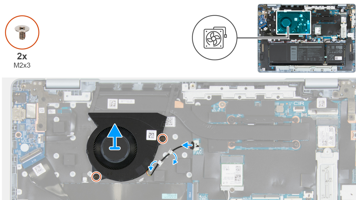
Figure 21. Removing the fan
