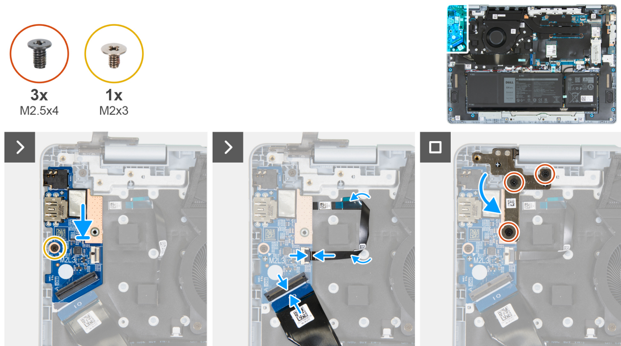
Figure 35. Installing the I/O board
