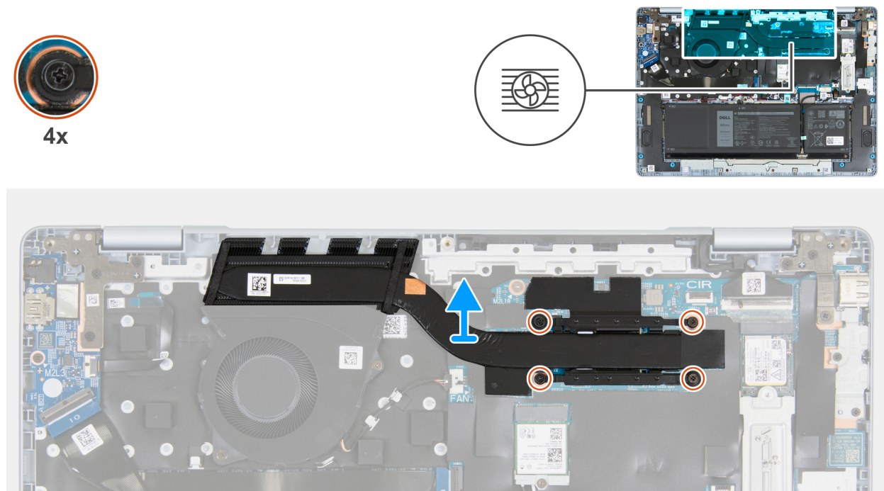
Figure 50. Removing the heat sink
