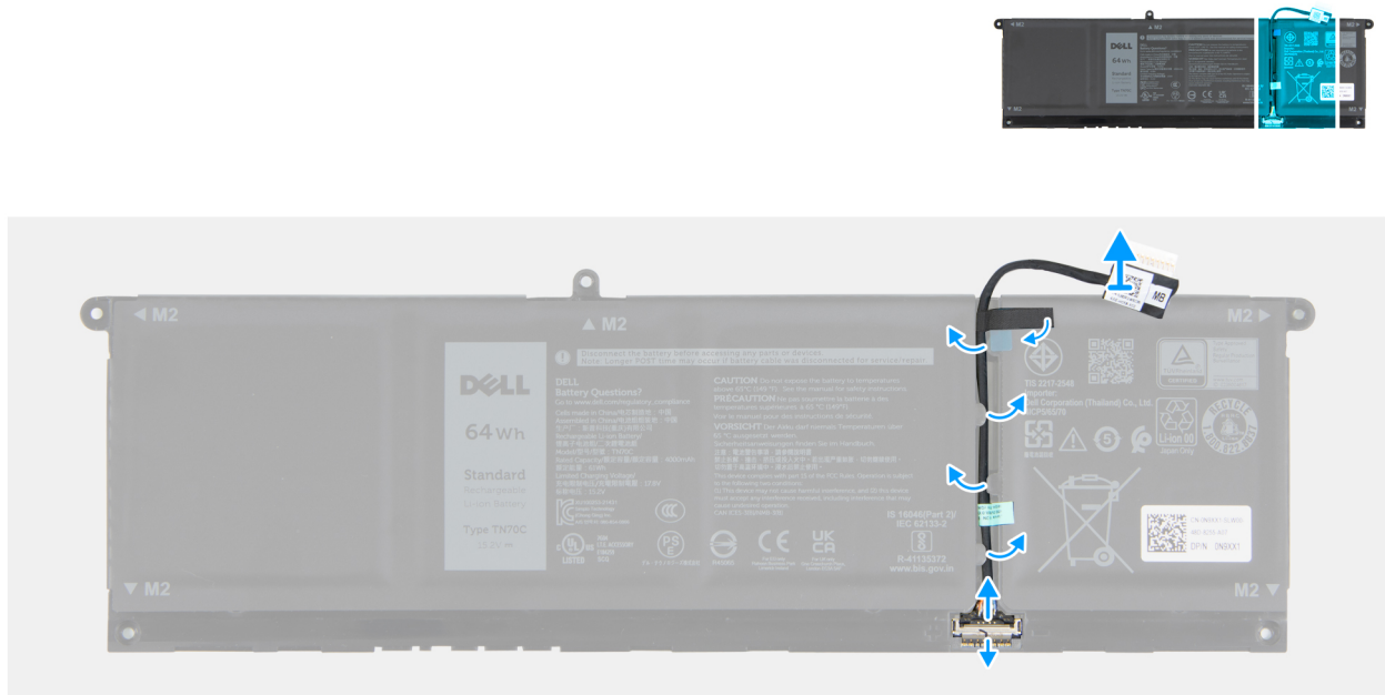
Figure 17. Removing the battery cable
