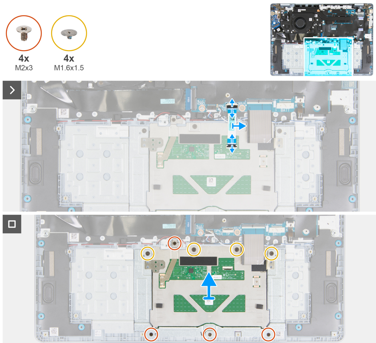
Figure 52. Removing the touchpad
