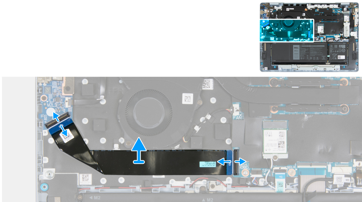
Figure 32. Removing the I/O-board cable
