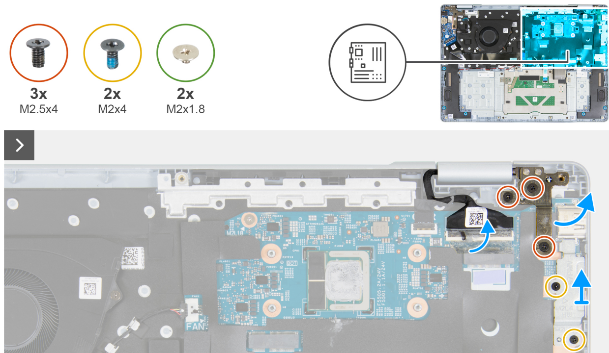
Figure 41. Removing the system board
