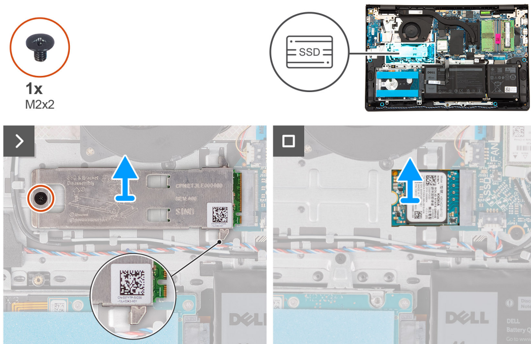
Figure 2. Removing the solid state drive
