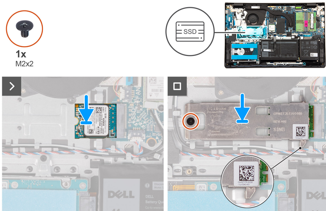
Figure 3. Installing the solid state drive
