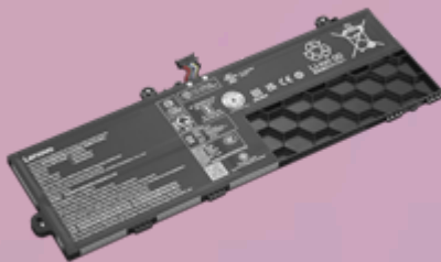
ThinkPad 3-cell 41Wh Li-ion Replacement Battery for X13 Gen6 4X51U04337
