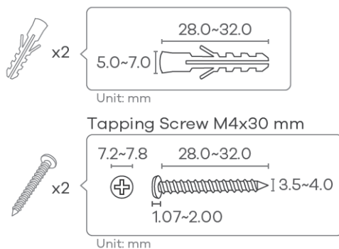
Figure 3 Screw Specifications
