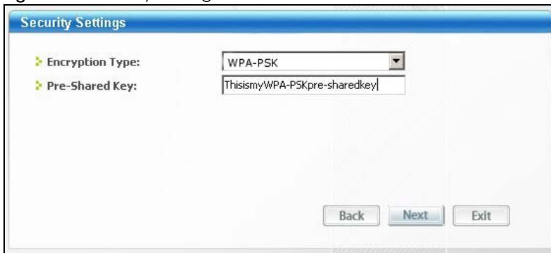
Figure 29 Security Settings
