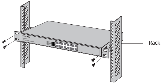
Figure 2-3 Rack Installation
