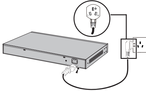
Figure 3-2 Connecting to the Ground
