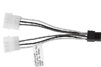
for 4-pin HDD power(from PSU)*2 to 6-pin
