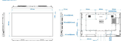
Philips 65BDL8051C Front view (mm)
