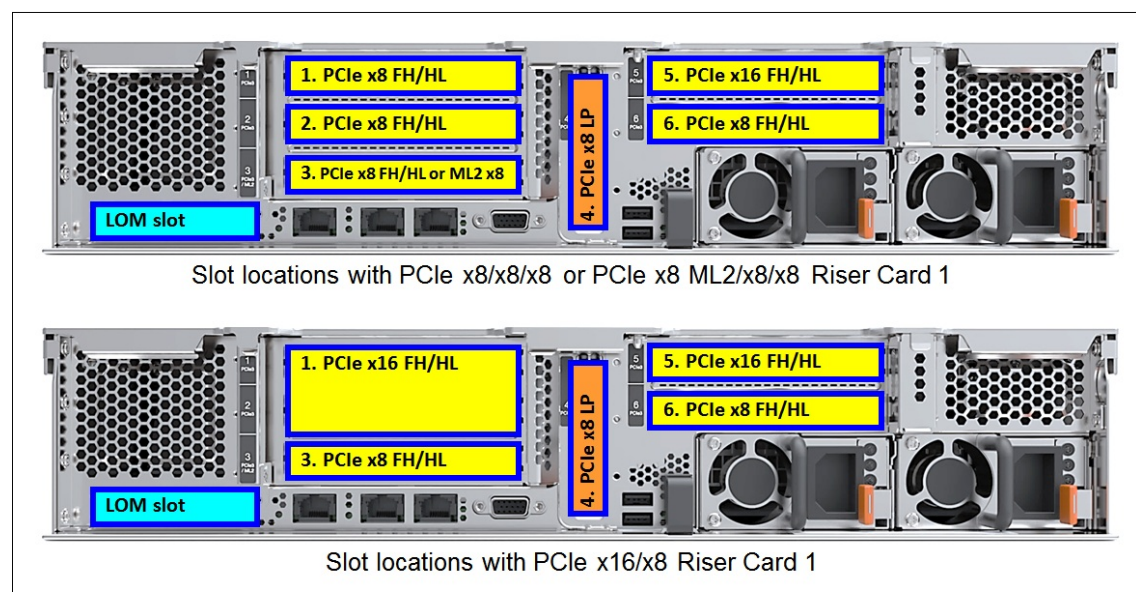
Figure 8. Slot locations
