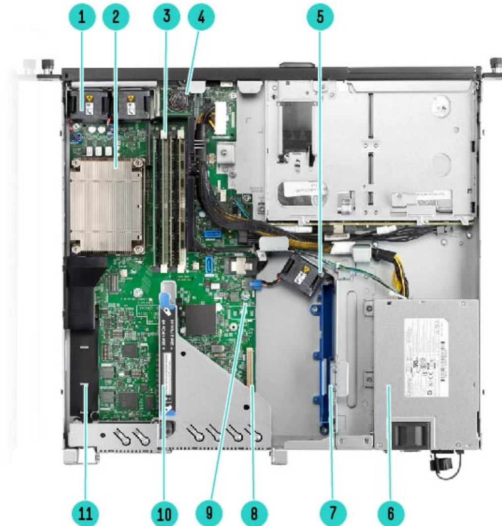
Internal View - Standard for all DL20 Gen10
