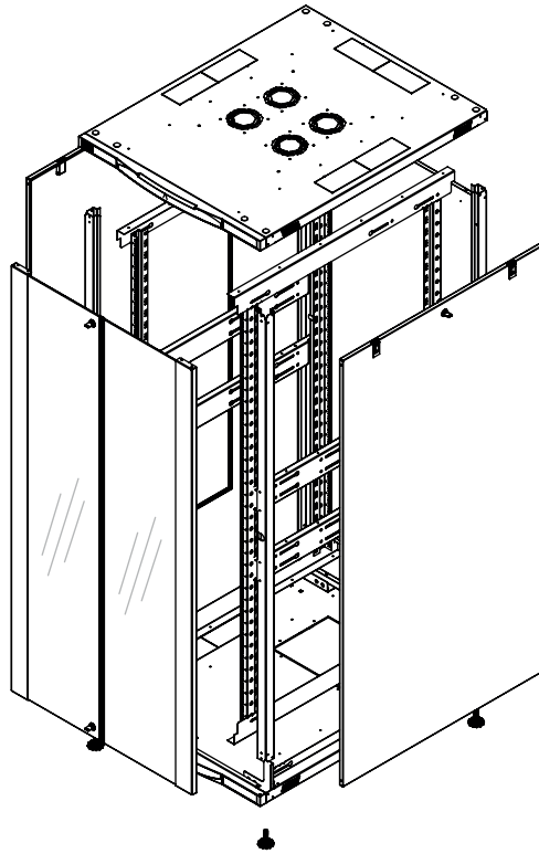
EXPLODED VIEW
