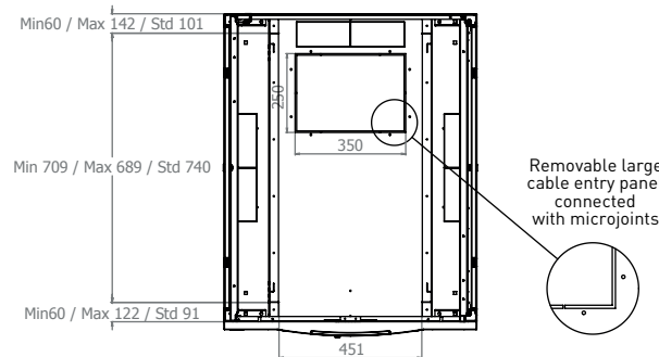
MAX/MIN/STD EQUIPMENT MOUNTING DISTANCE
