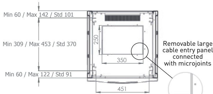
MAX/MIN/STD EQUIPMENT MOUNTING DISTANCE
