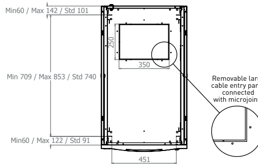
MAX/MIN/STD EQUIPMENT MOUNTING DISTANCE
