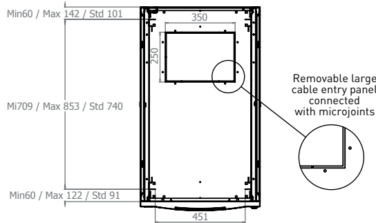
MAX/MIN/STD EQUIPMENT MOUNTING DISTANCE
