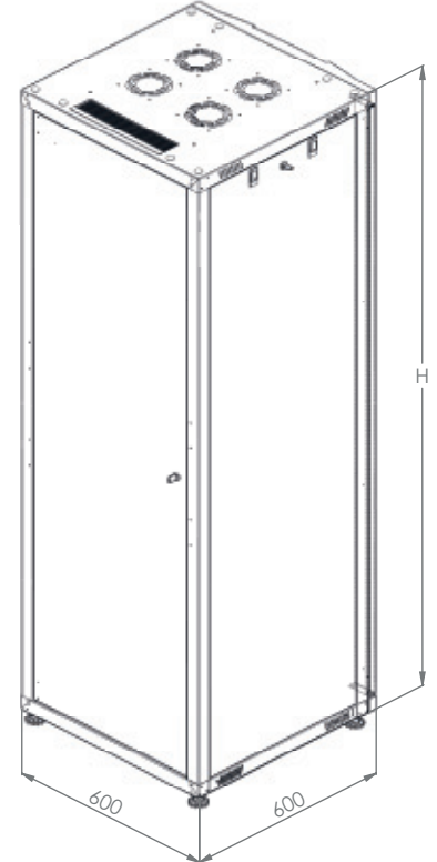
REAR VIEW
