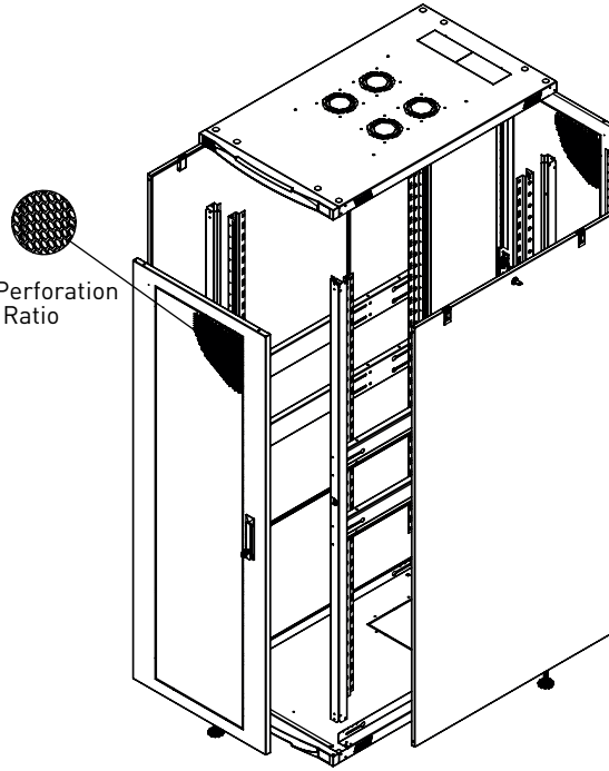
EXPLODED VIEW
