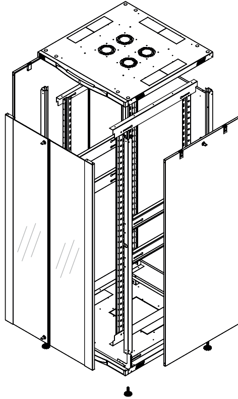
EXPLODED VIEW
