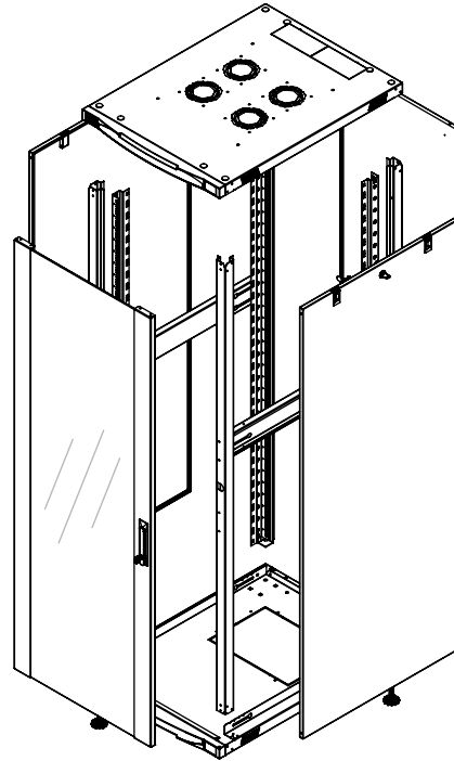
EXPLODED VIEW
