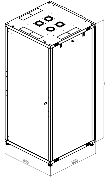
REAR VIEW
