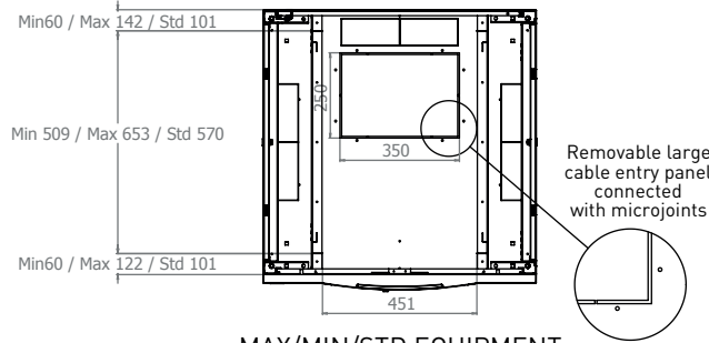
MAX/MIN/STD EQUIPMENT MOUNTING DISTANCE
