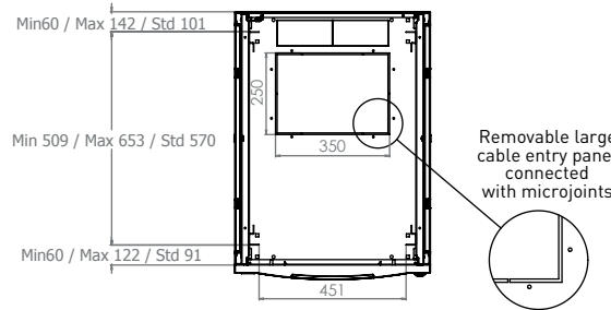
MAX/MIN/STD EQUIPMENT MOUNTING DISTANCE
