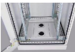
Sealed Cable Entry From Bottom
