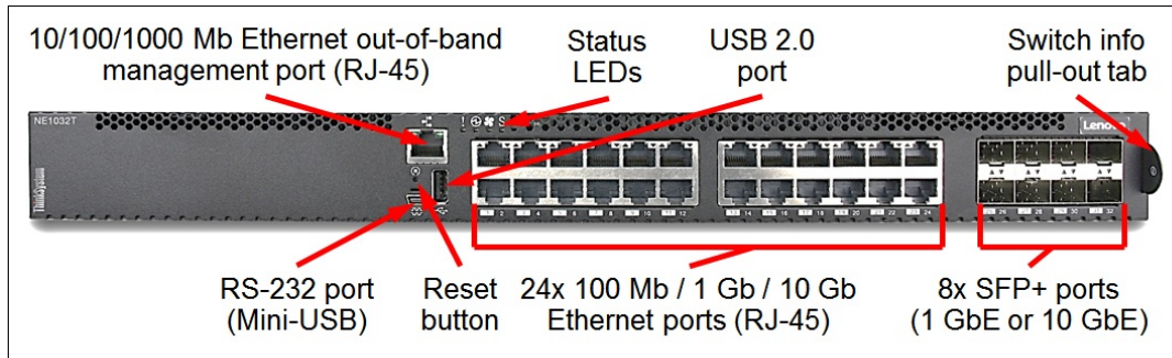
Figure 2. Front panel of the NE1032T RackSwitch
